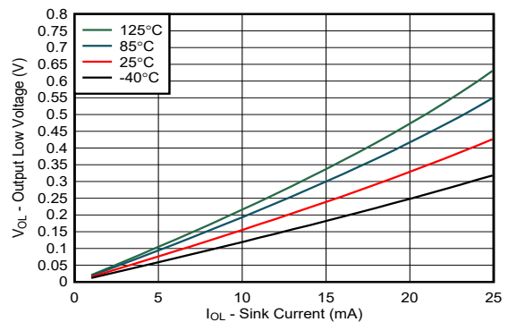
FIG 6-8. I/O Sink Current vs Output Low Voltage for Different Temperature ( T_A ) for V_{CC} = 2.3\text{ V}
