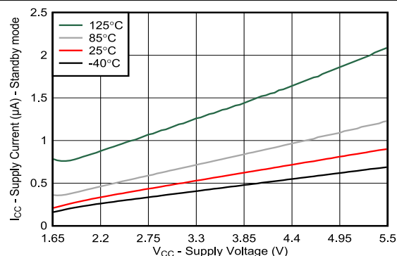
FIG 6-1. Supply Current (Standby) vs Supply Voltage for Different Temperature ( T_A )
