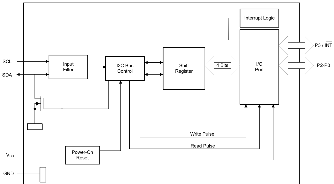
8-1. Logic Diagram
