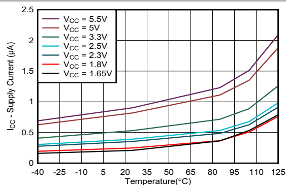
FIG 6-3. Standby Supply Current vs Temperature for Different Supply Voltage ( V_{CC} )
