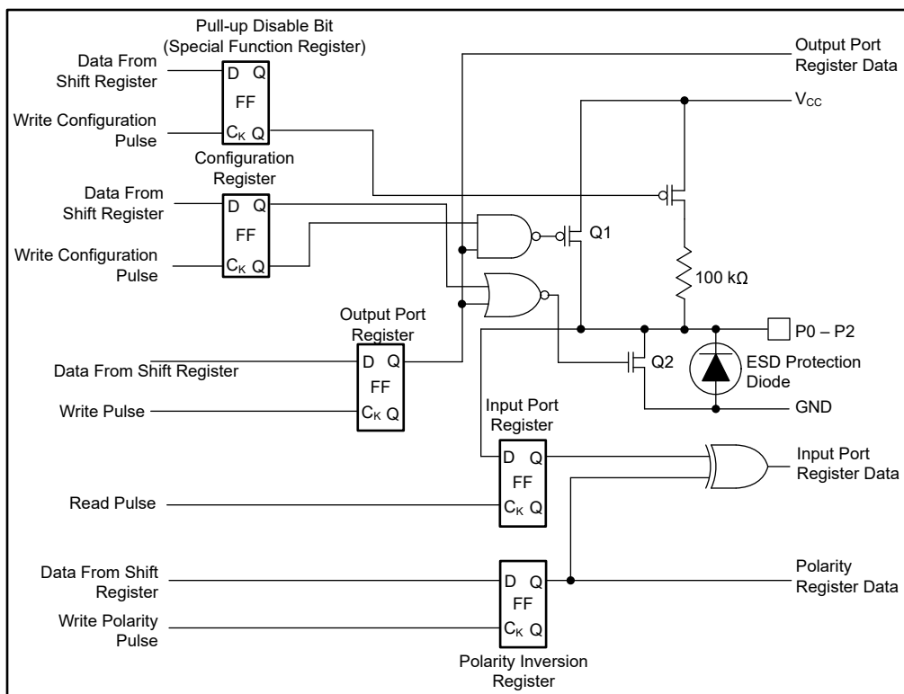
8-2. Simplified Schematic Of P0 To P2
