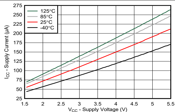
FIG 6-2. Supply Current vs Supply Voltage for Different Temperature ( T_A )
