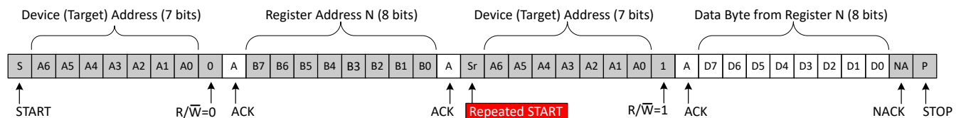
FIG 8-8. Read from Register
