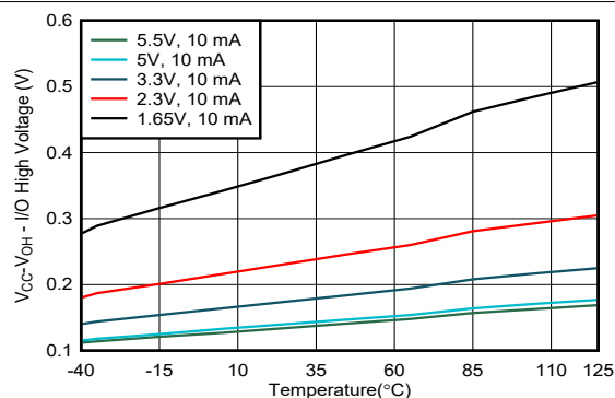
FIG 6-5. V_{CC} - V_{OH} Voltage vs Temperature for Different V_{CC}
