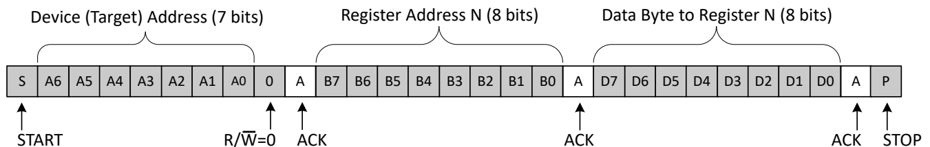
8-6. Write to Register
