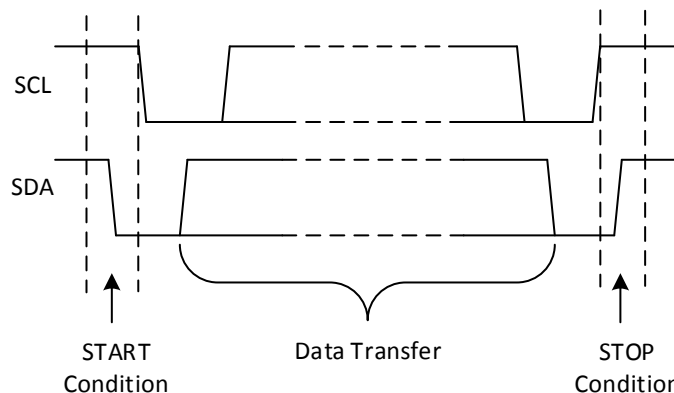
☒ 8-4. Definition of Start and Stop Conditions
