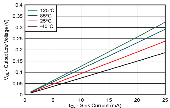
FIG 6-10. I/O Sink Current vs Output Low Voltage for Different Temperature ( T_A ) for V_{CC} = 5.5\text{ V}
