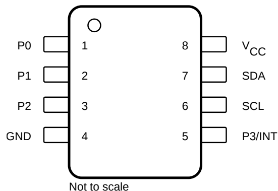
图 5-2. DGK Package, 8-Pin VSSOP, Top View
