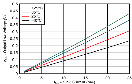
FIG 6-9. I/O Sink Current vs Output Low Voltage for Different Temperature ( T_A ) for V_{CC} = 3.3\text{ V}
