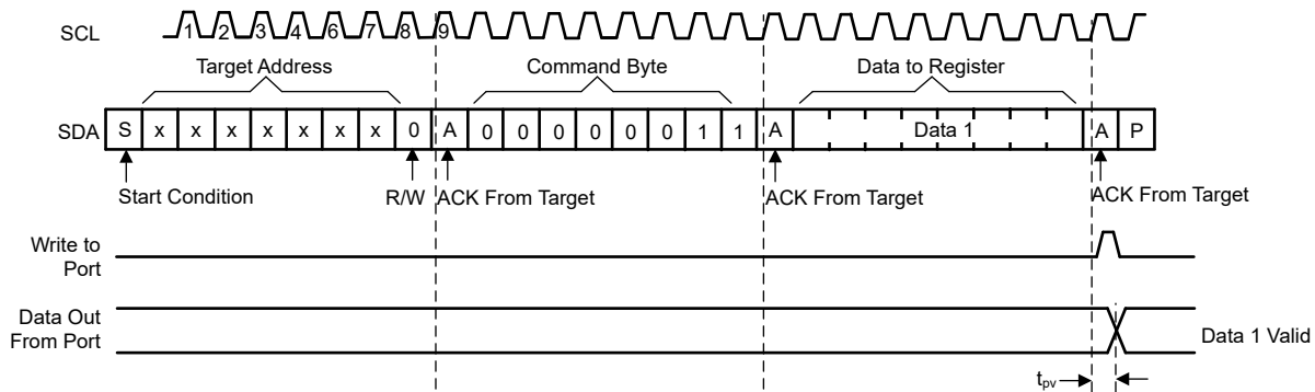
FIG 8-7. Write to Output Port Register
