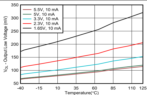
FIG 6-6. V_{OL} vs Temperature for Different V_{CC}
