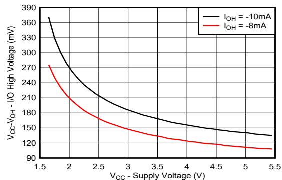
FIG 6-7. V_{CC} - V_{OH} Voltage at 25^\circ\text{C} for Different V_{CC}
