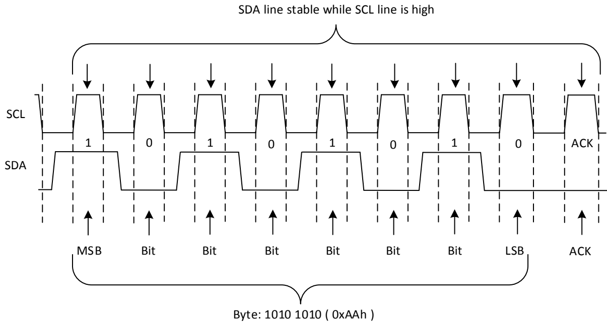
8-5. Bit Transfer
