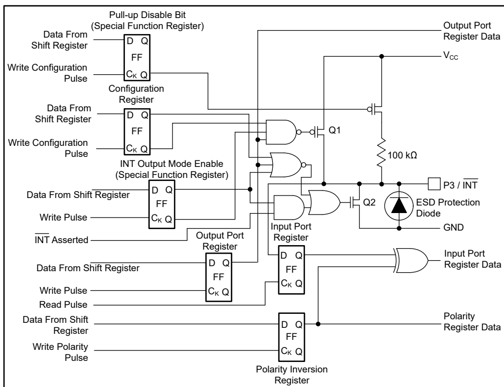
8-3. Simplified Schematic Of P3 / INT
