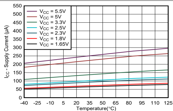
FIG 6-4. Supply Current vs Temperature for Different Supply Voltage ( V_{CC} )
