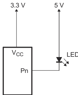
8-3. Device Supplied by Lower Voltage
