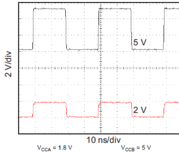
✎ 12. Level-Translation of a 2.5-MHz Signal
