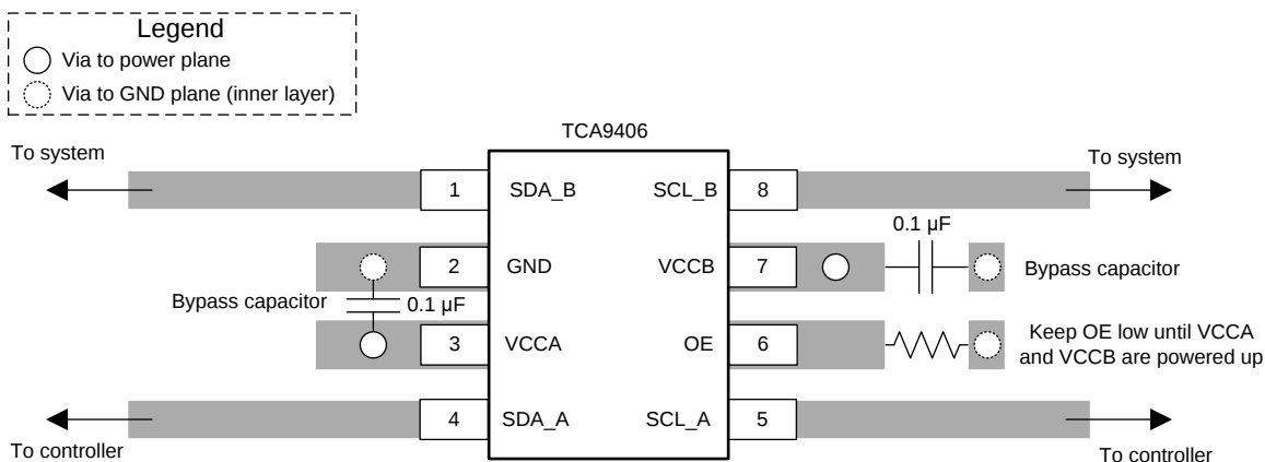
✎ 13. TCA9406 Layout Example
