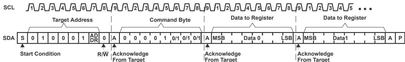
Figure 8-8. Write to Configuration or Polarity Inversion Registers
