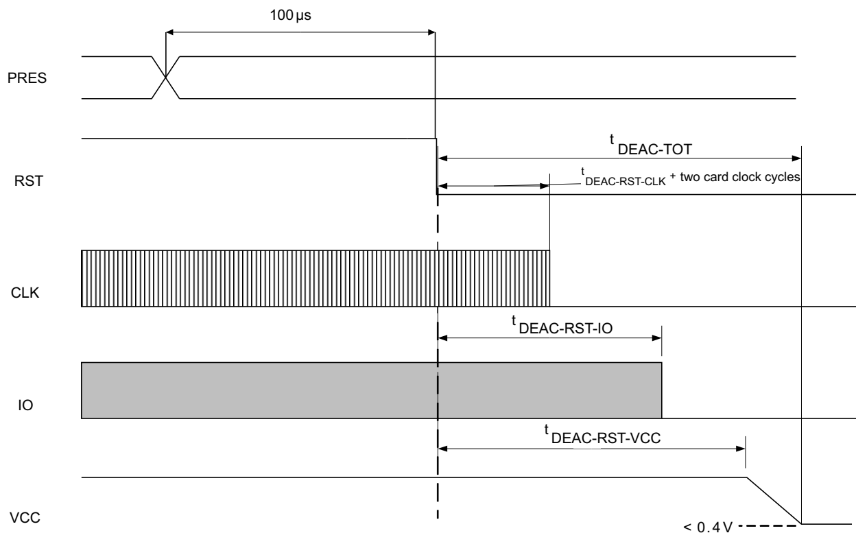
Figure 7. Deactivation Sequence
