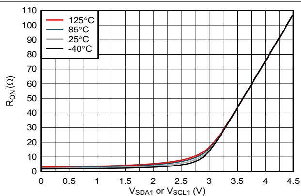
図 5-2. On-Resistance ( R_{ON} ) vs Input Voltage ( V_{SDA1} or V_{SCL1} )
