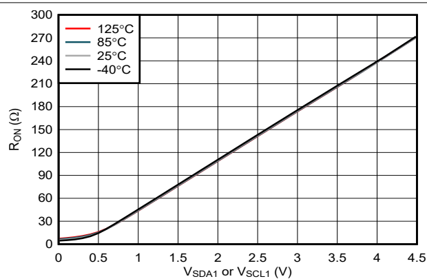
図 5-1. On-Resistance ( R_{ON} ) vs Input Voltage ( V_{SDA1} or V_{SCL1} )
