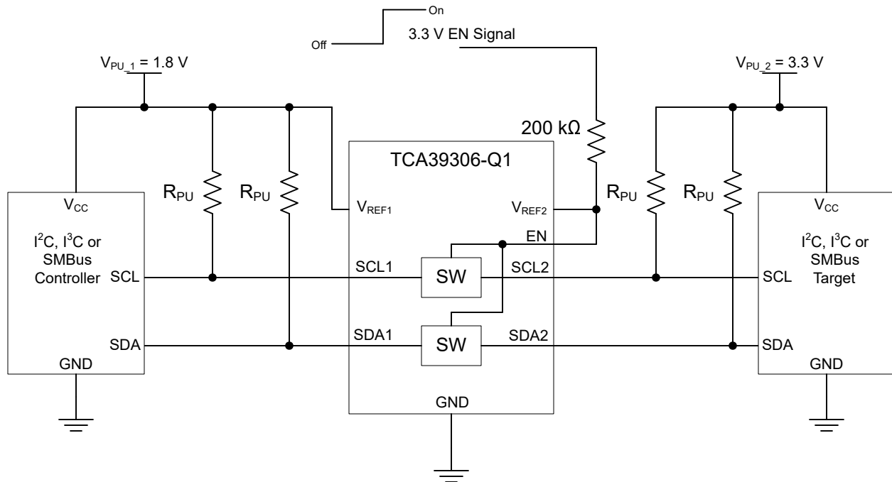
図 8-2. Typical Application Circuit (Switch Enable Control)
