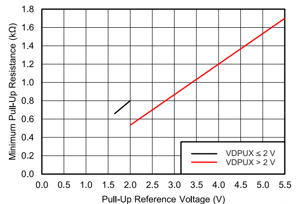
8-4. Minimum Pullup Resistance ( R_{p(min)} ) vs Pullup Reference Voltage ( V_{DPUX} )
