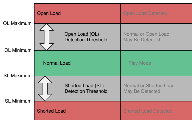
FIG 9-6. DC Load Diagnostic Reporting Thresholds
