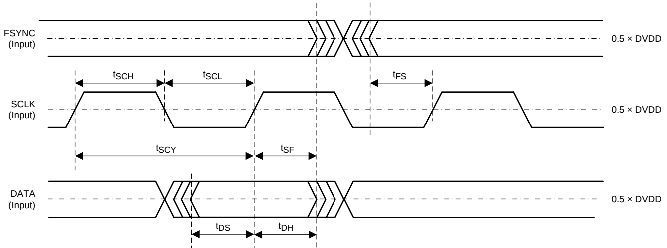
FIG 16. Serial Audio Timing
