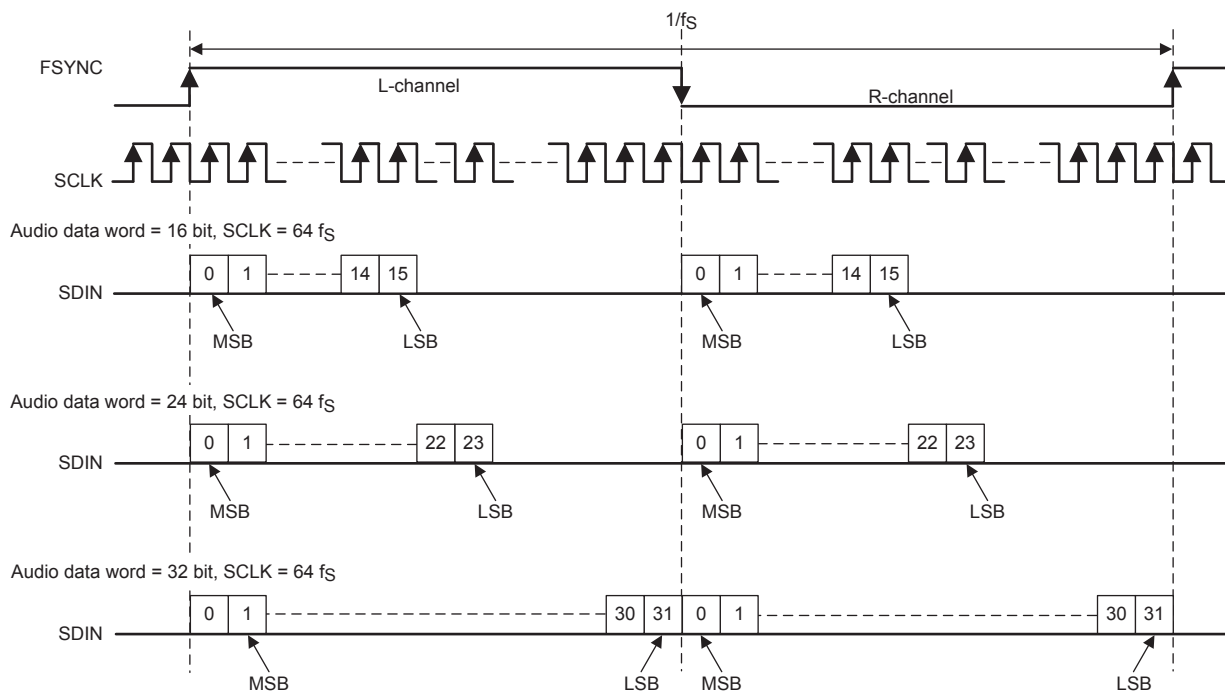
FIG 17. Left-Justified Audio Data Format
