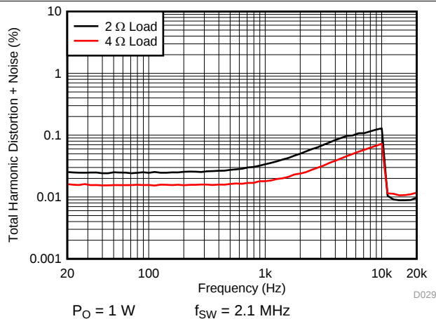
Figure 12. PBTL THD+N vs Frequency
