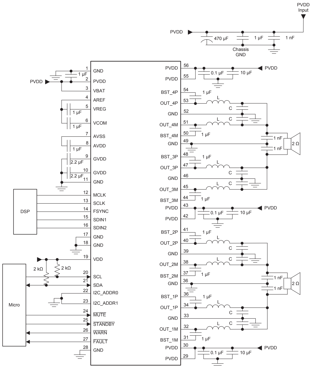
FIG 62. TAS6424L-Q1 Typical 2-Channel PBTL Application Schematic
