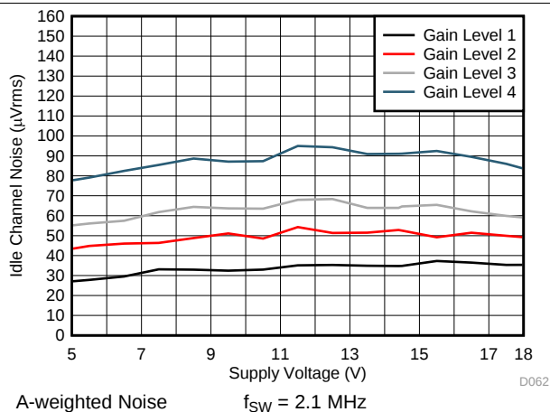
Figure 8. Noise vs Supply voltage
