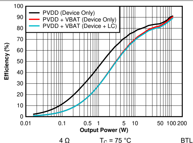
7-7. Efficiency vs Output Power - 14.4 V - 4 \Omega (Zoomed)
