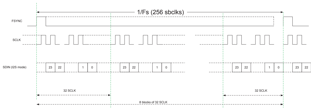
Figure 9-5. TDM8 Audio Data Format
