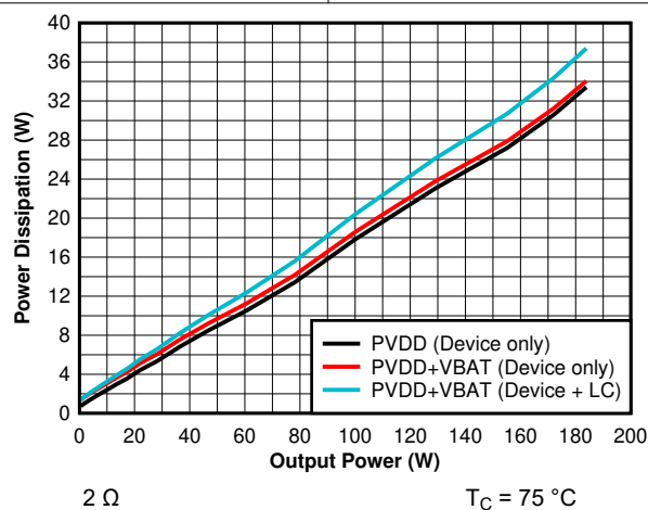
7-27. Power Dissipation vs Output Power - 2 \Omega - 384 kHz
