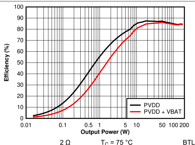
7-26. Efficiency vs Output Power - 2 \Omega - 384 kHz (Zoomed)
