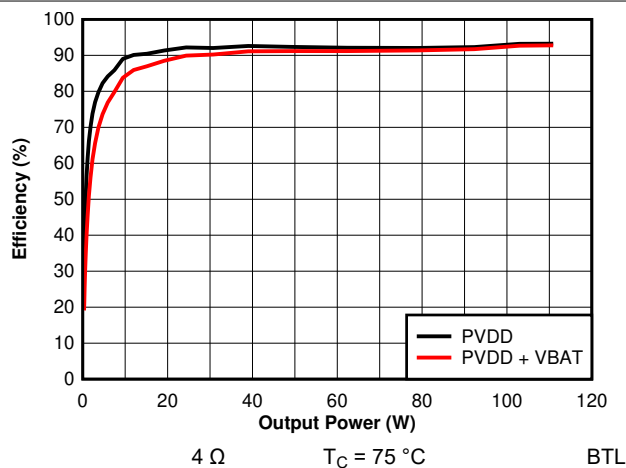
7-22. Efficiency vs Output Power - 4 \Omega - 384 kHz
