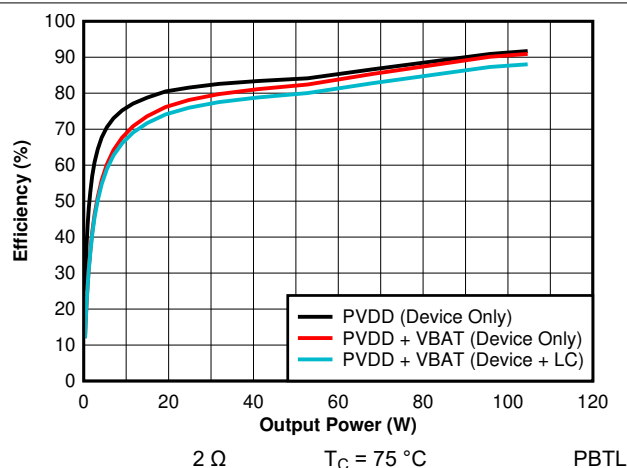
7-33. Efficiency vs Output Power - PBTB - 2 ohm
