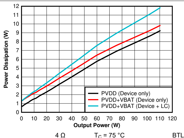
7-24. Power Dissipation vs Output Power - 4 \Omega - 384 kHz
