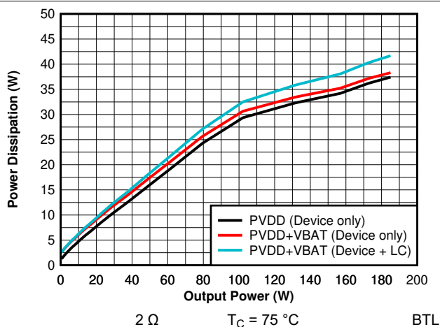
7-11. Power Dissipation vs Output Power - 14.4 V - 2 \Omega
