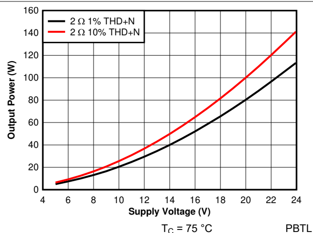
7-32. Output Power vs Supply Voltage - PBTB
