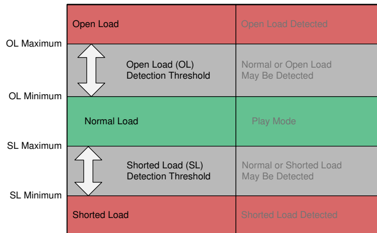
FIG 9-7. DC Load Diagnostic Reporting Thresholds
