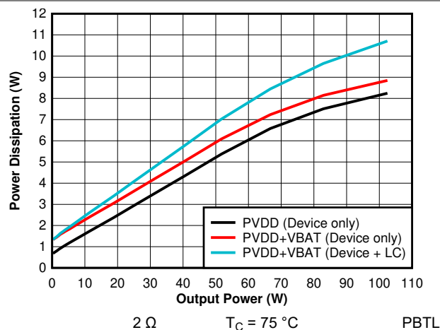
7-42. Power Dissipation vs Output Power - PBTL - 2 \Omega - 384kHz
