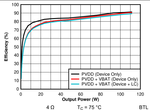
Figure 7-6. Efficiency vs Output Power - 14.4 V - 4 Ω
