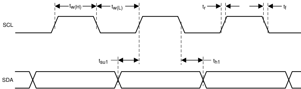
FIG 9-9. SCL and SDA Timing
