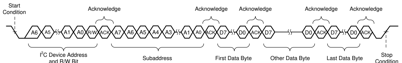
FIG 9-11. Sequential Write Transfer
