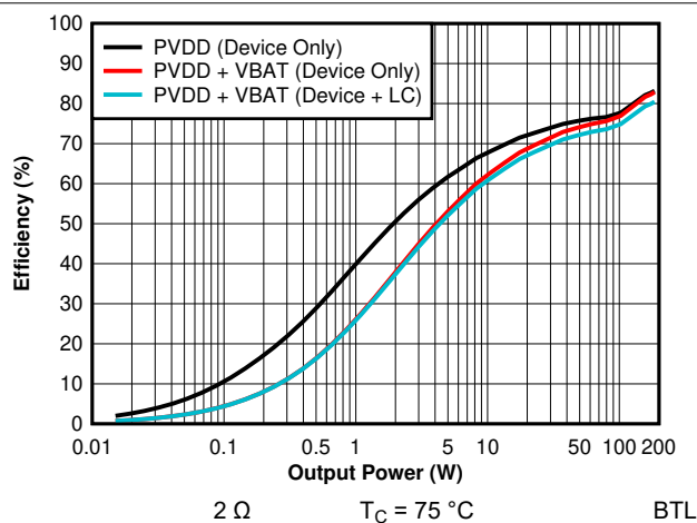
7-10. Efficiency vs Output Power - 14.4 V - 2 \Omega (Zoomed)
