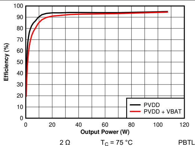
7-40. Efficiency vs Output Power - PBTL - 2 \Omega - 384 kHz
