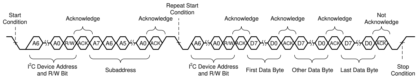
FIG 9-13. Sequential Read Transfer
