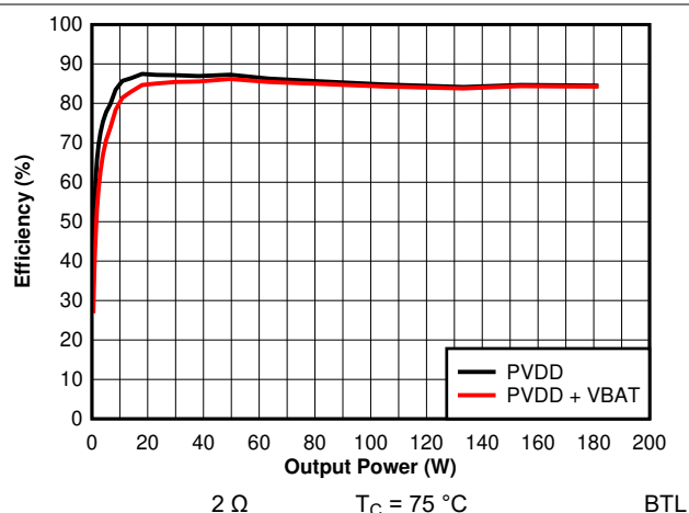
7-25. Efficiency vs Output Power - 2 \Omega - 384 kHz
