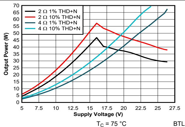
Figure 7-5. Output Power vs Supply Voltage
