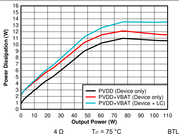
7-8. Power Dissipation vs Output Power - 14.4 V - 4 \Omega
