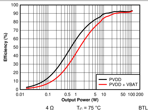
7-23. Efficiency vs Output Power - 4 \Omega - 384 kHz (Zoomed)
