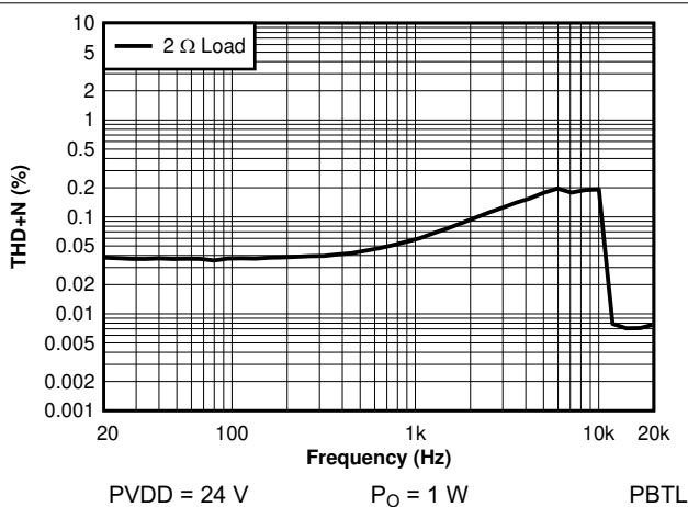
7-31. THD+N vs Frequency - PBTB - 24 V
