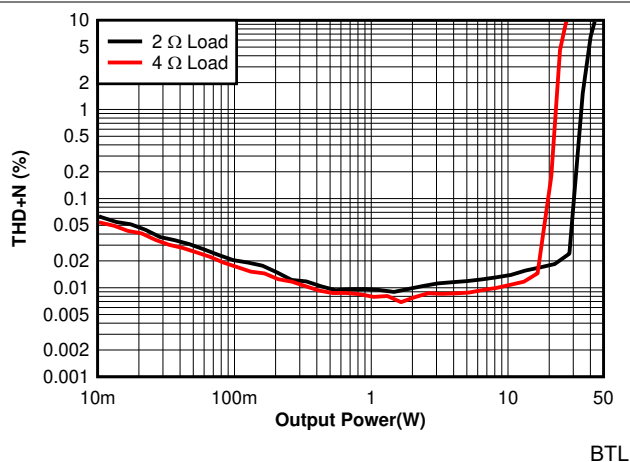
7-19. THD+N vs Power - 384 kHz
