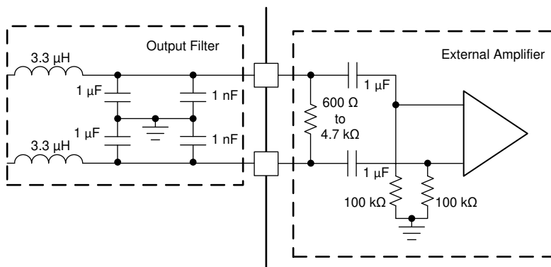
FIG 10-1. External Amplifier Input Configuration for Line Driver
