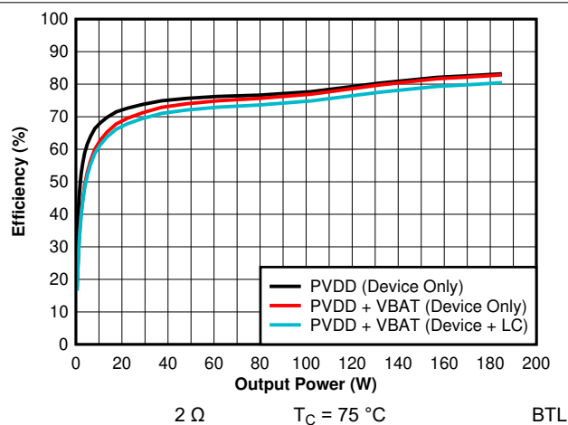
7-9. Efficiency vs Output Power - 14.4 V - 2 \Omega
