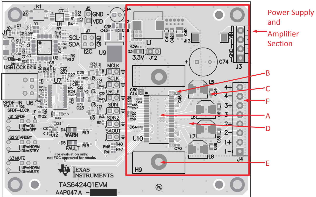
Figure 12-1. EVM Layout
