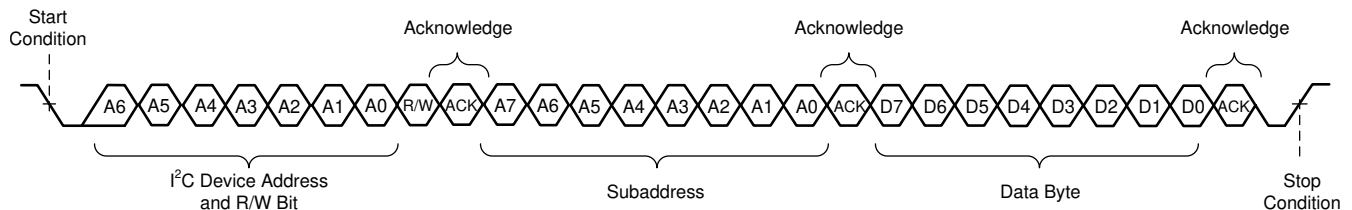
FIG 9-10. Random Write Transfer
