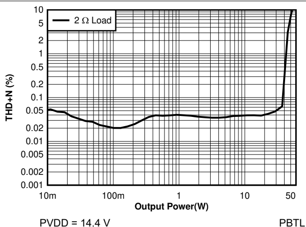
7-28. THD+N vs Power - PBTB - 14.4V
