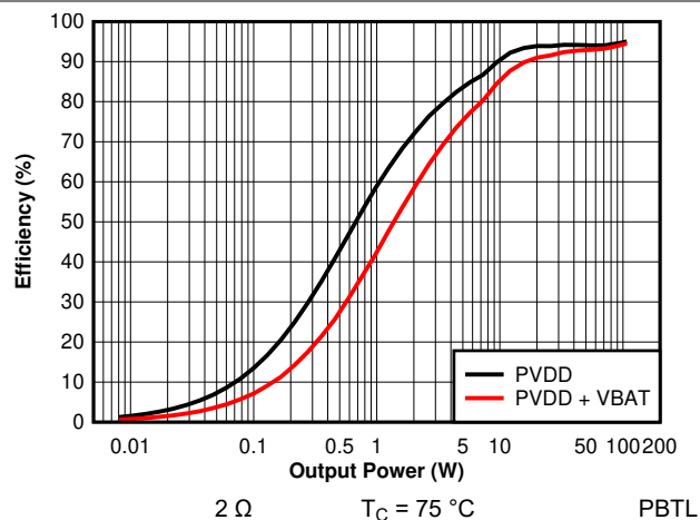
7-41. Efficiency vs Output Power - PBTL - 2 \Omega - 384 kHz (Zoomed)
