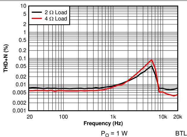
7-20. THD+N vs Frequency - 384 kHz
