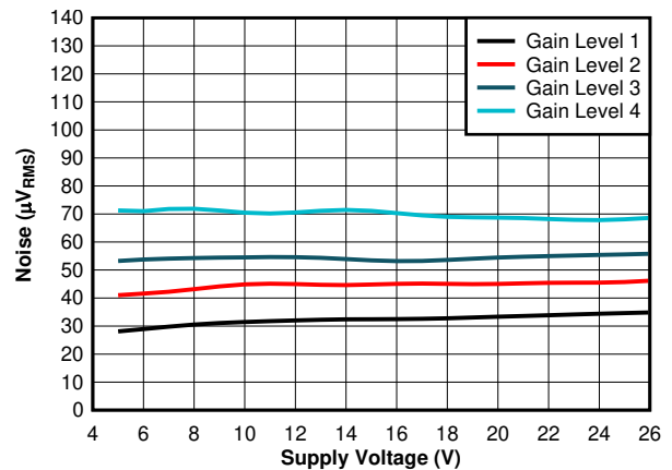
7-14. Noise vs Supply Voltage
