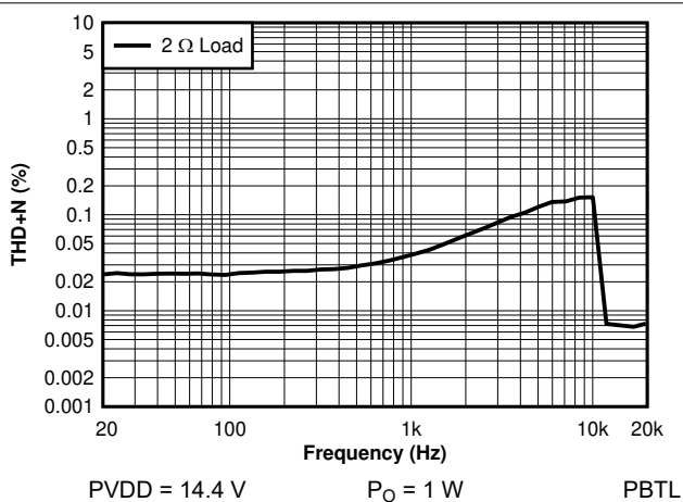
7-30. THD+N vs Frequency - PBTB - 14.4 V
