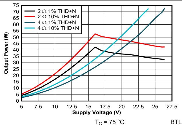
7-21. Output Power vs Supply Voltage - 384 kHz
