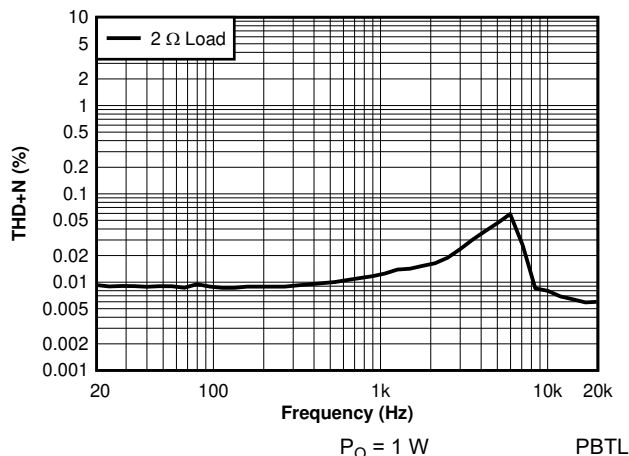
7-38. THD+N vs Frequency - PBTL - 384 kHz
