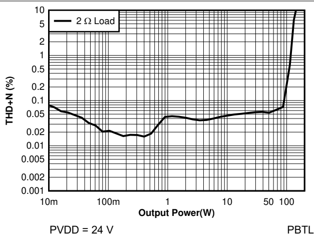
7-29. THD+N vs Power - PBTB - 24 V
