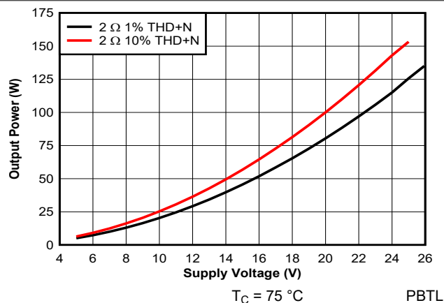
7-39. Output Power vs Supply Voltage - PBTL - 384 kHz
