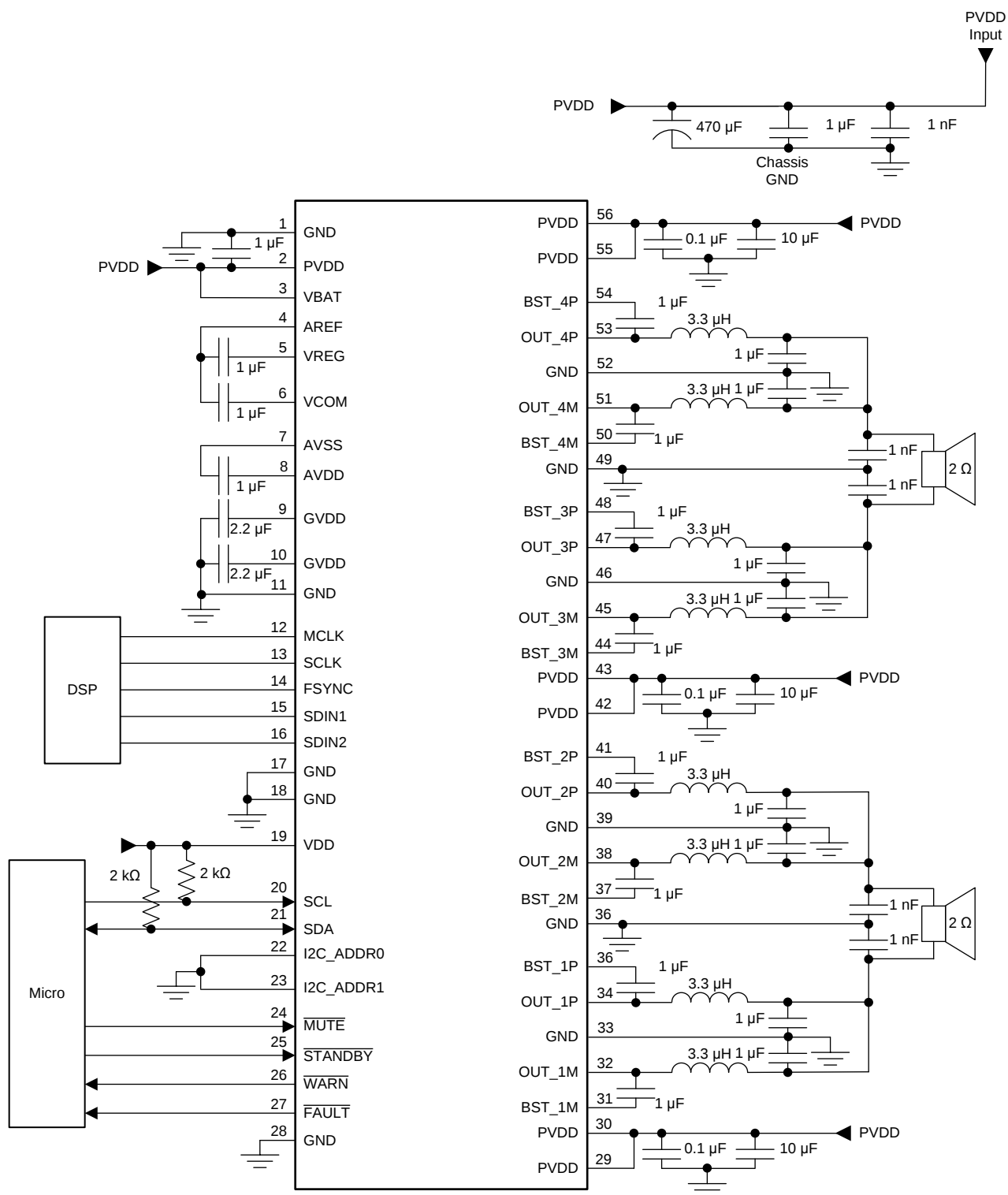
82. 2-Channel PBTL Application Schematic
