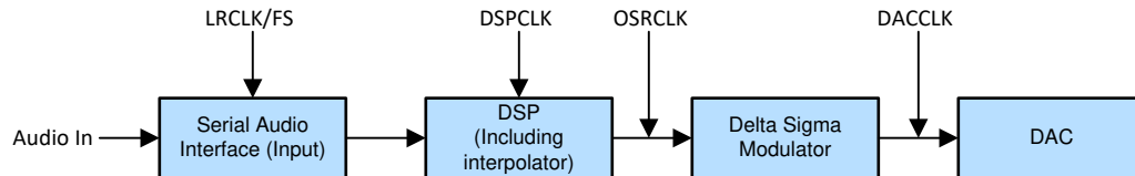
图 7-1. Audio Flow with Respective Clocks
