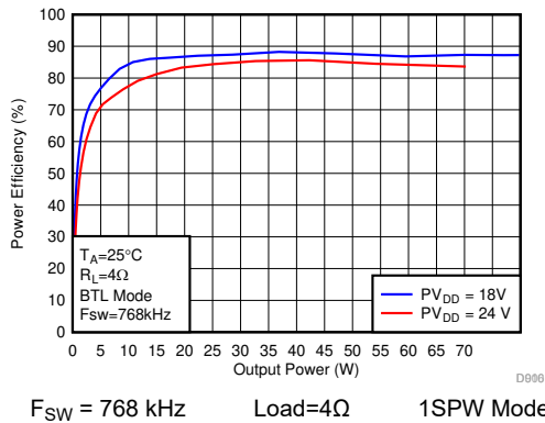
6-3. Efficiency vs Output Power-BTL
