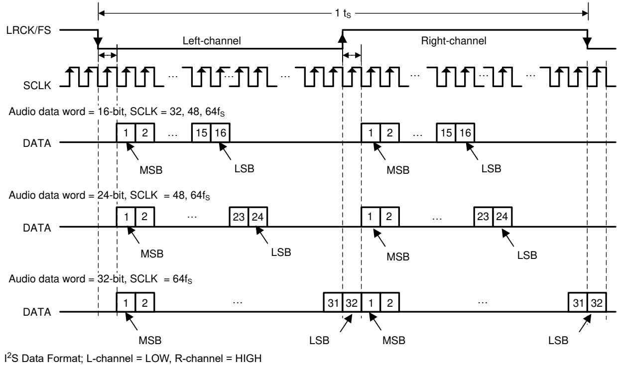
FIG 7-3. I²S Audio Data Format
