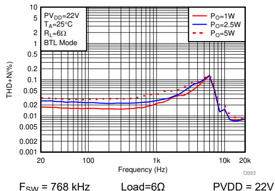
6-22. THD+N vs Frequency-BTL
