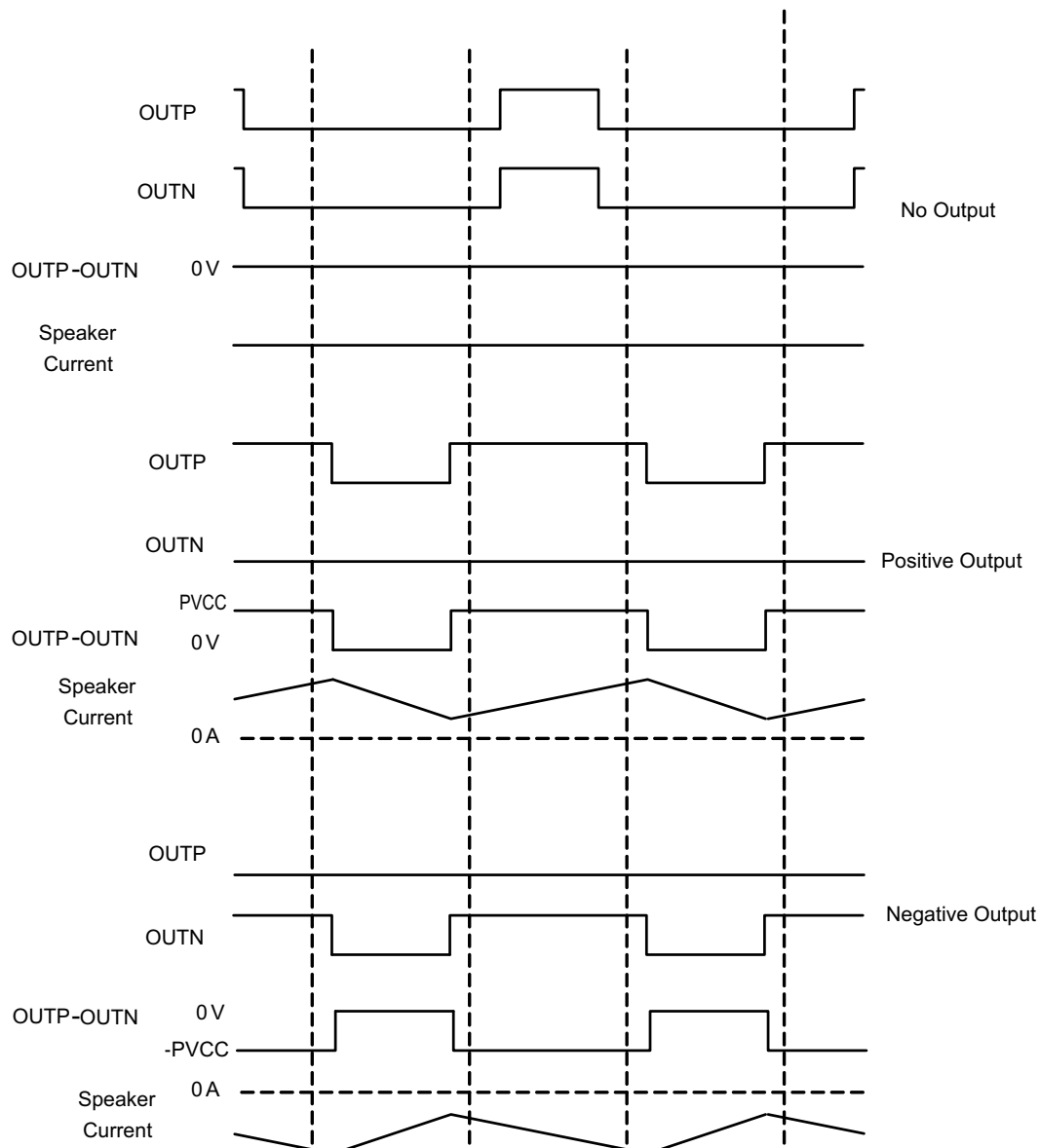
7-10. 1SPW Mode Modulation
