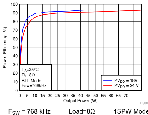
6-5. Efficiency vs Output Power-BTL
