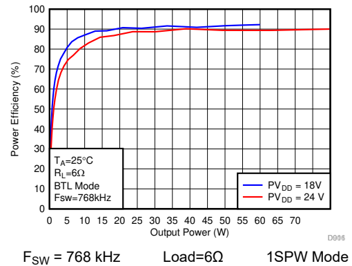
6-4. Efficiency vs Output Power-BTL
