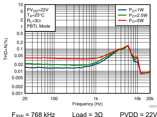
6-50. THD+N vs Frequency
