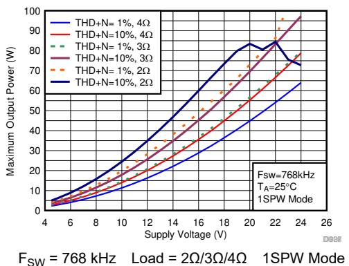
Figure 6-37. Output Power vs PVDD
