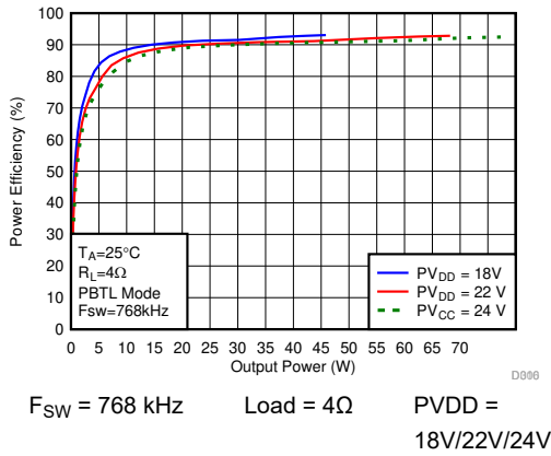
Figure 6-33. Efficiency vs Output Power
