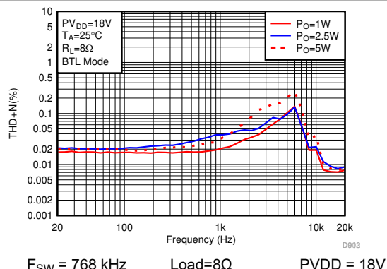
6-24. THD+N vs Frequency-BTL
