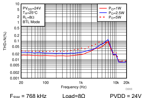
6-26. THD+N vs Frequency-BTL
