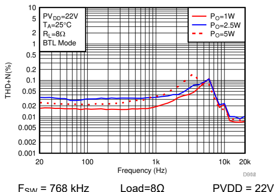
6-25. THD+N vs Frequency-BTL
