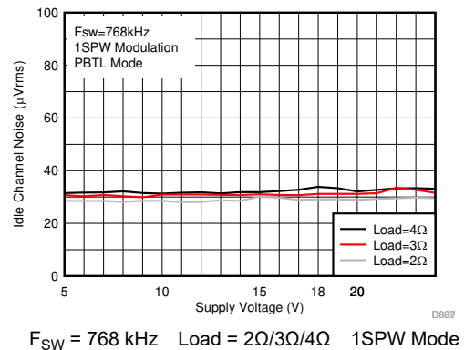
Figure 6-36. Idle Channel Noise vs PVDD
