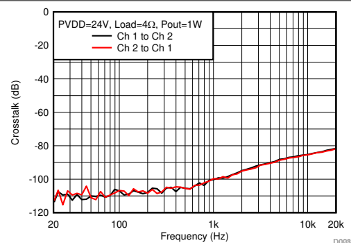
6-28. Crosstalk vs Frequency-BTL
