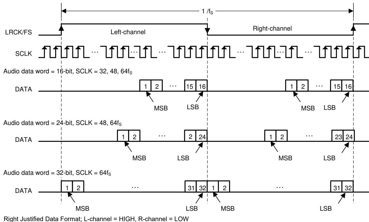
FIG 7-4. Right Justified Audio Data Format
