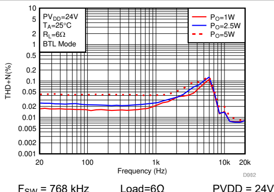
6-23. THD+N vs Frequency-BTL
