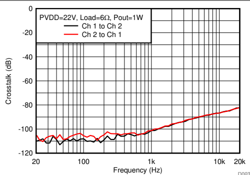
6-27. Crosstalk vs Frequency-BTL
