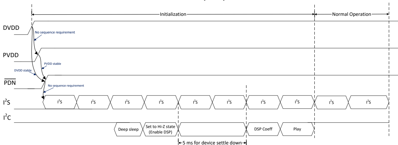
✎ 7-15. Startup sequence
