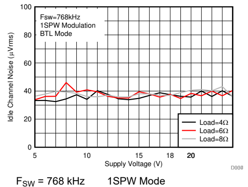
6-6. Idle Channel Noise vs Supply Voltage
