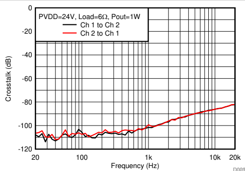
6-29. Crosstalk vs Frequency-BTL
