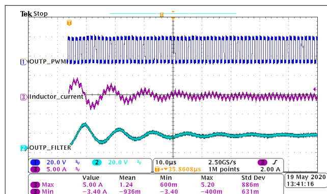
Figure 8-3. Start-up Current (Fsw = 768 kHz, LC filter = 4.7 µH + 0.68 µF, PVDD = 24 V, BD Modulation)
