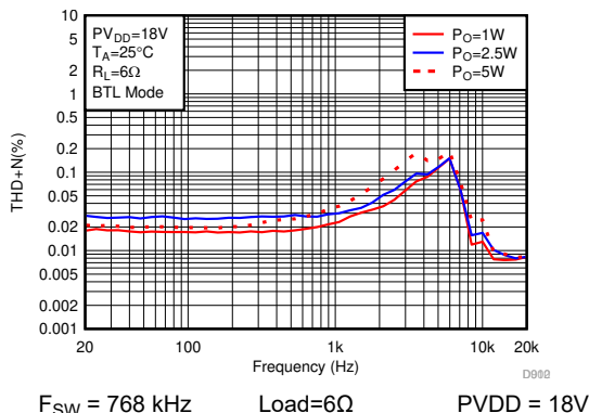
6-21. THD+N vs Frequency-BTL
