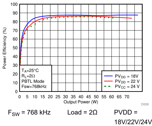
Figure 6-35. Efficiency vs Output Power
