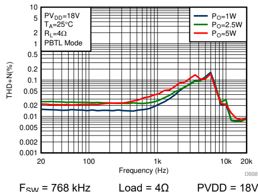
6-46. THD+N vs Frequency
