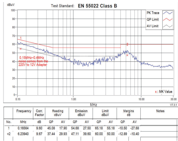
8-6. Conducted Emission with Ferrite Bead Filter - Neutral
