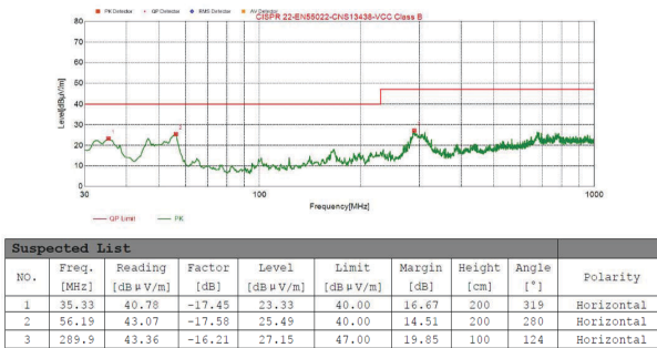
8-7. Radiated Emission with Ferrite Bead Filter - Horizontal
