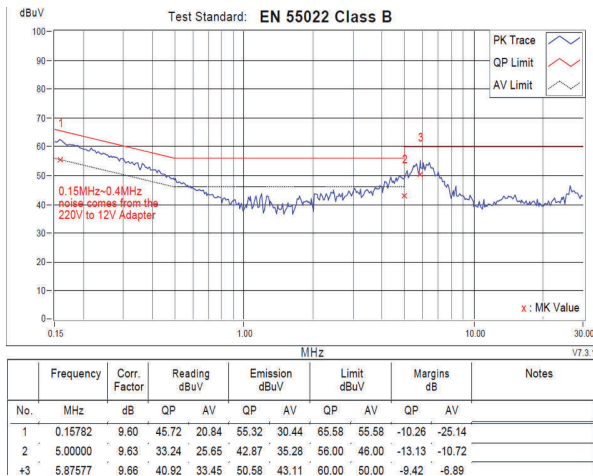
8-5. Conducted Emission with Ferrite Bead Filter - Line
