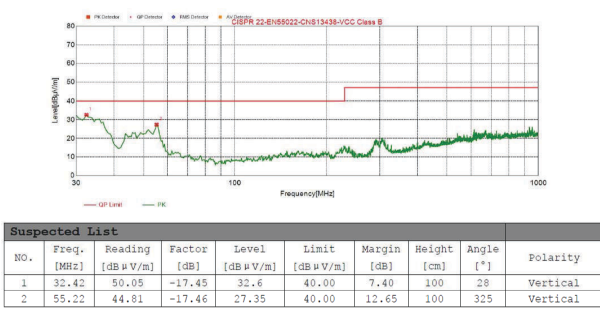
8-8. Radiated Emission with Ferrite Bead Filter - Vertical
