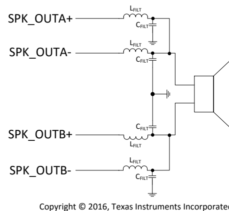
Figure 79. Post-Filter PBTL
