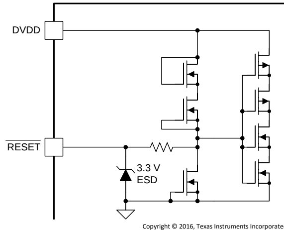
Figure 17. RESET Pin
