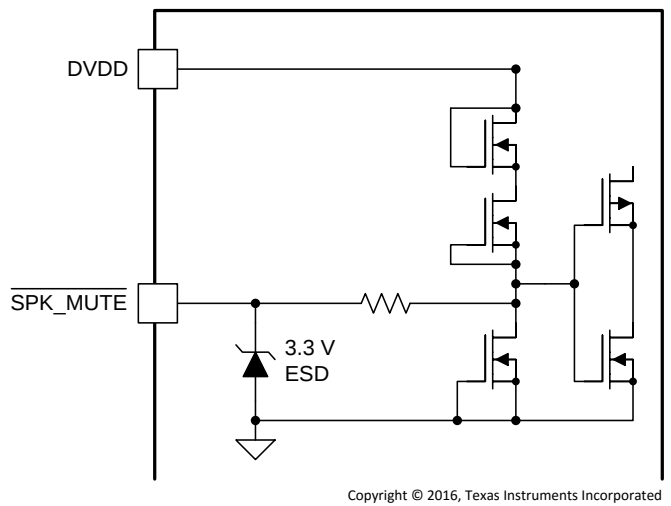
Figure 12. \overline{\text{SPK\_MUTE}} Pin
