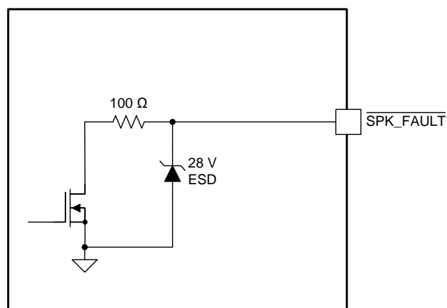
Figure 16. SPK_FAULT Pin
