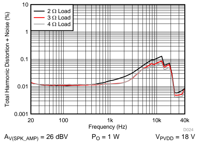
Figure 46. THD+N vs Frequency – PBTL
