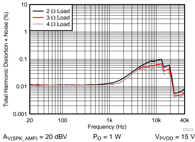
Figure 45. THD+N vs Frequency – PBTL
