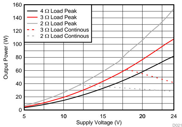
Figure 43. Output Power vs PVDD – PBTL
