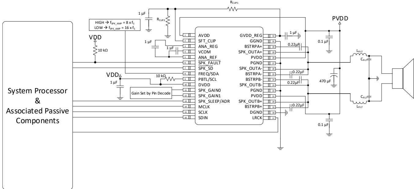
Figure 65. Mono PBTL using Hardware Control, 32 Pin DAP Package Option
