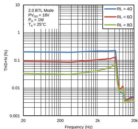
FIG 23. Total Harmonic Distortion vs Frequency
