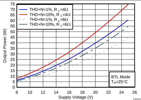
FIG 18. Output Power vs Supply Voltage
