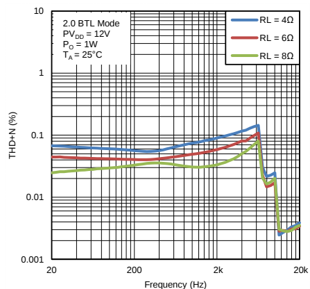
FIG 22. Total Harmonic Distortion vs Frequency
