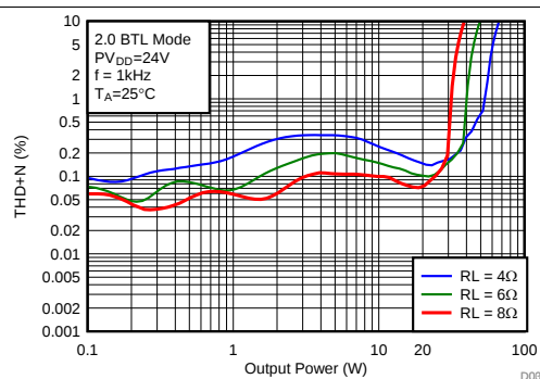
FIG 21. Total Harmonic Distortion + Noise vs Output Power
