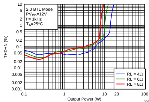
FIG 19. Total Harmonic Distortion + Noise vs Output Power
