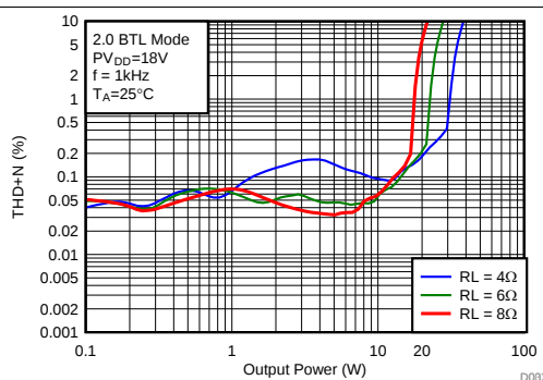
FIG 20. Total Harmonic Distortion + Noise vs Output Power
