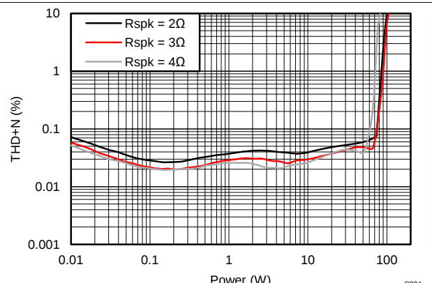
Figure 50. THD+N vs Power – PBTL
