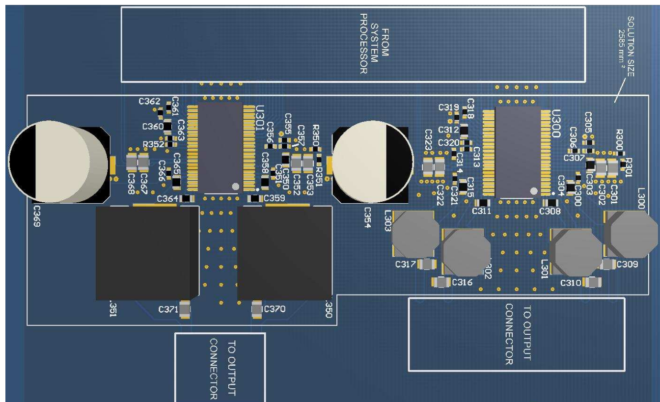
Figure 90. 2.1 (Stereo BTL + Mono PBTL) 3-D View
