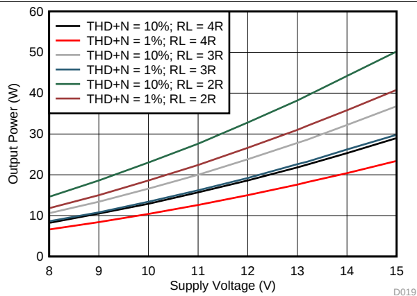
Figure 23. Output Power vs PVDD - PBTL
