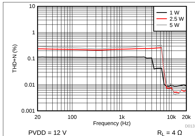
Figure 17. THD+N vs Frequency - PBTL
