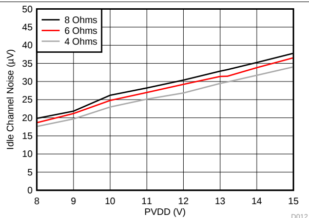
Figure 6. Idle Channel Noise vs Supply Voltage - BTL
