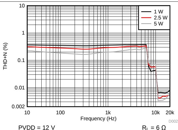
Figure 8. THD+N vs Frequency - BTL
