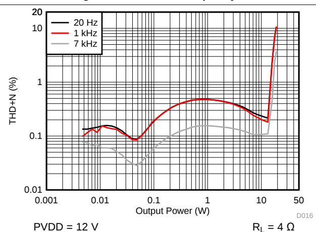
Figure 20. THD+N vs Output Power - PBTL
