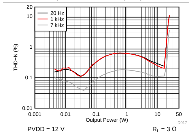
Figure 21. THD+N vs Output Power - PBTL
