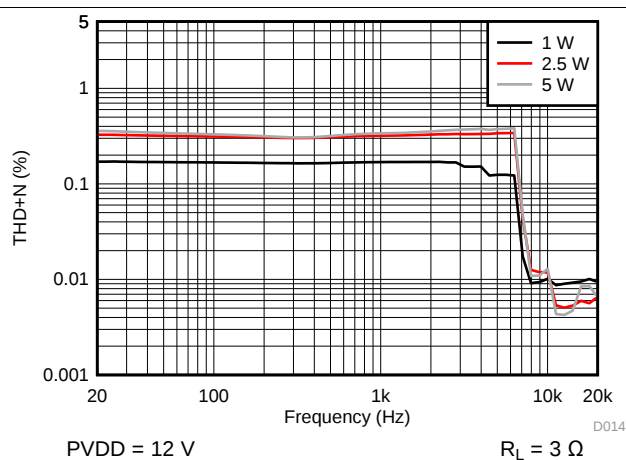
Figure 18. THD+N vs Frequency - PBTL
