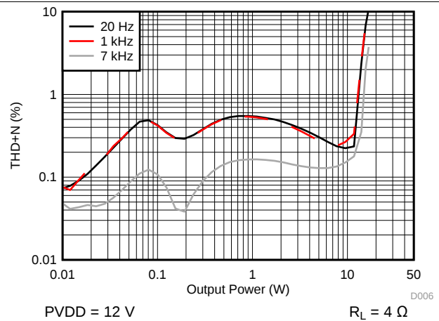
Figure 12. THD+N vs Output Power - BTL
