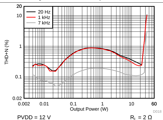
Figure 22. THD+N vs Output Power - PBTL
