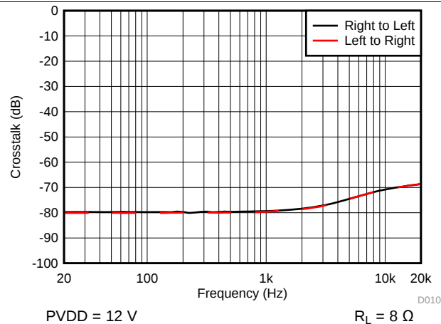
Figure 15. Crosstalk vs Frequency - BTL
