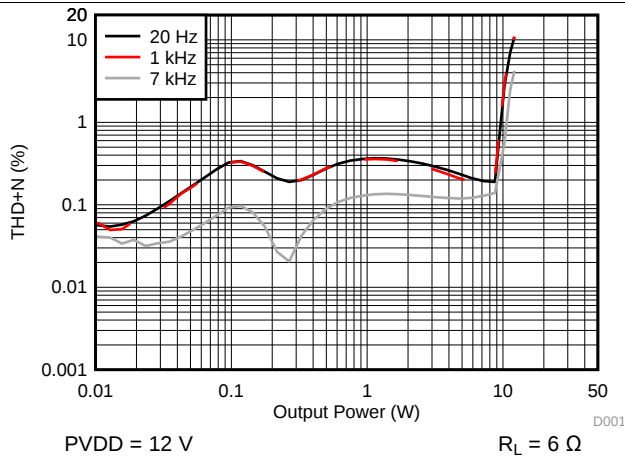
Figure 11. THD+N vs Output Power - BTL
