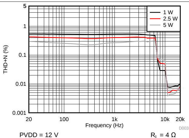
Figure 9. THD+N vs Frequency - BTL
