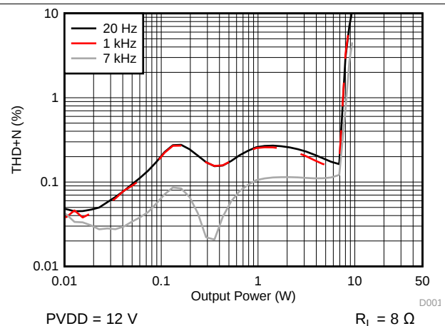
Figure 10. THD+N vs Output Power - BTL
