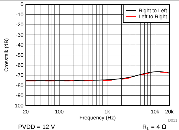
Figure 16. Crosstalk vs Frequency - BTL
