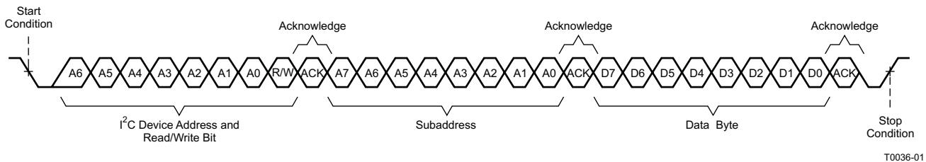
Figure 33. Single-Byte Write Transfer
