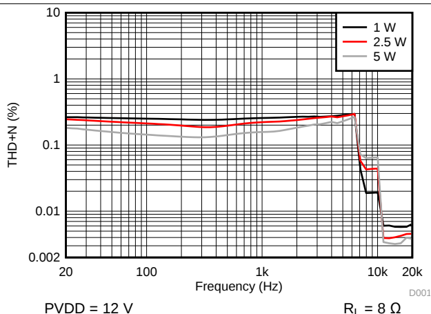
Figure 7. THD+N vs Frequency - BTL
