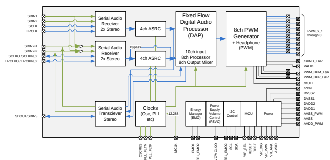
Block Diagram
