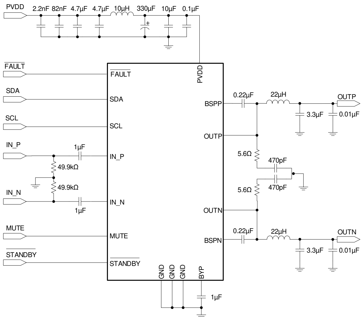
図 8-1. TAS5431-Q1 Typical Application Schematic
