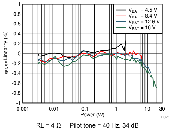
FIG 6-21. I_{\text{SENSE}} Gain Linearity vs Output Power
