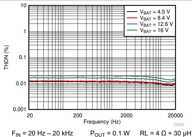
图 6-5. THD+N vs Frequency
