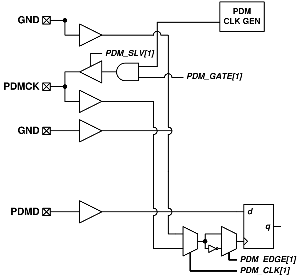
図 8-7. PDM Data and Clock Input Block Diagram
