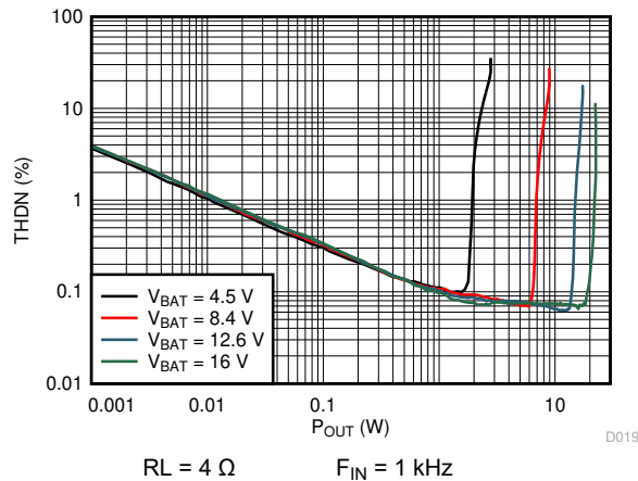
FIG 6-19. I_{\text{SENSE}} THD+N vs Output Power
