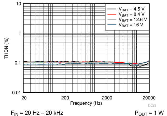
FIG 6-22. I_{\text{SENSE}} THD+N vs Frequency
