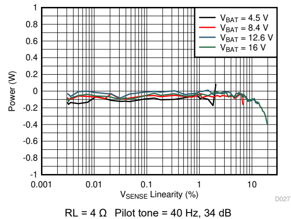
FIG 6-26. Output Power vs V_{\text{SENSE}} Linearity
