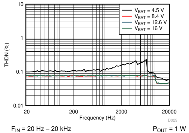
FIG 6-28. V_{\text{SENSE}} THD+N vs Frequency
