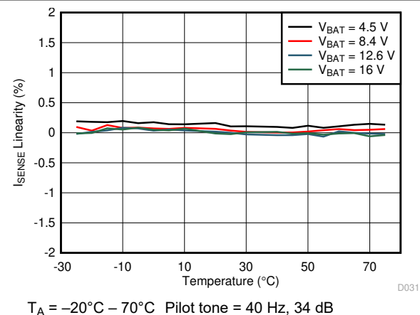
FIG 6-30. I_{\text{SENSE}} Gain Deviation vs Temperature
