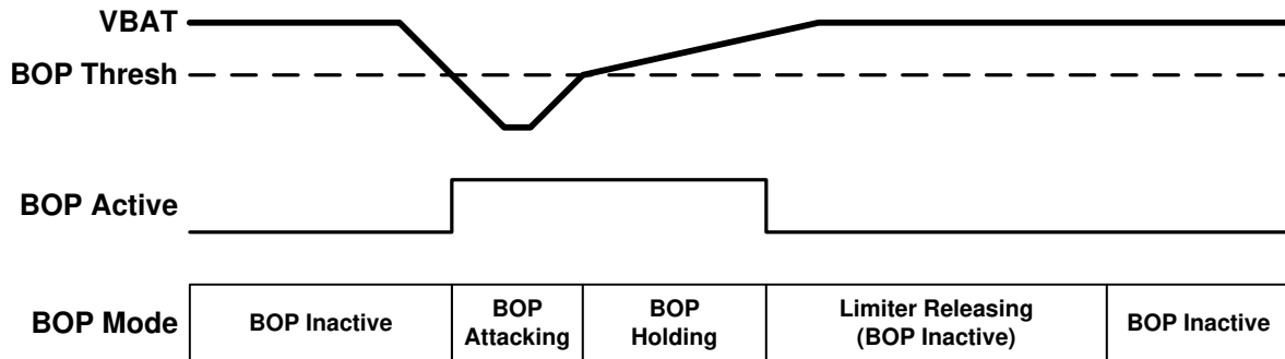
図 8-16. Brown Out Prevention Event
