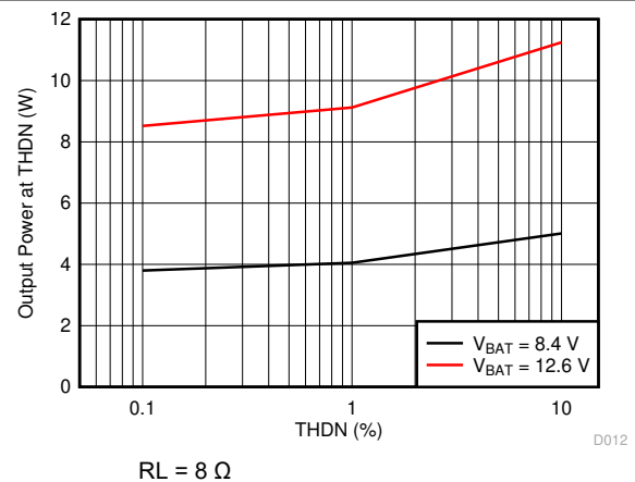
Figure 6-12. Max Output Power vs THD+N
