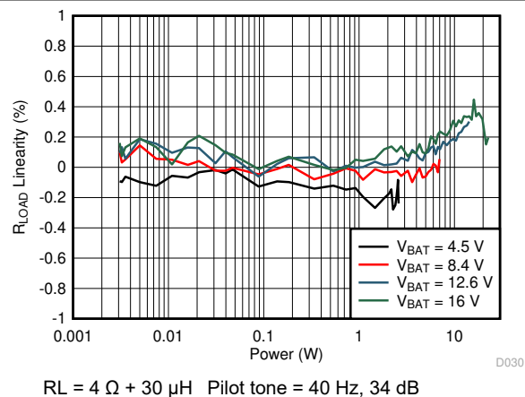
FIG 6-29. V/I_{\text{SENSE}} Gain Linearity vs Output Power
