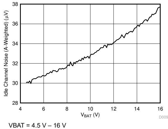
Figure 6-9. Idle Channel Noise (A-Weighted) vs V_{\text{BAT}}
