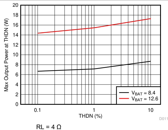
Figure 6-11. Max Output Power vs THD+N
