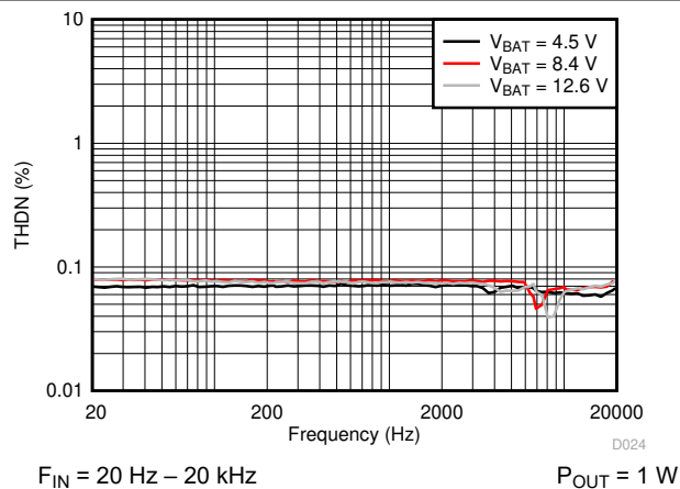
FIG 6-23. I_{\text{SENSE}} THD+N vs Frequency
