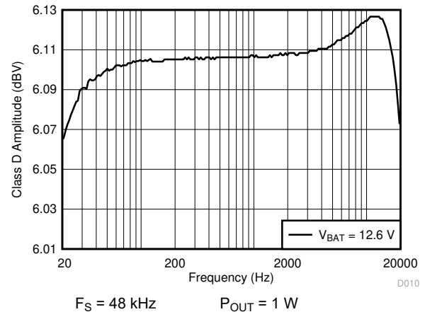
Figure 6-10. Amplitude vs Frequency
