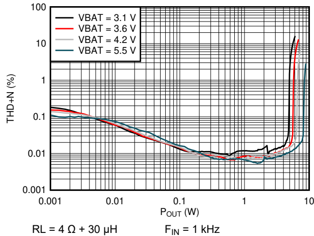
図 5-5. THD+N vs Output Power (DSBGA Package)
