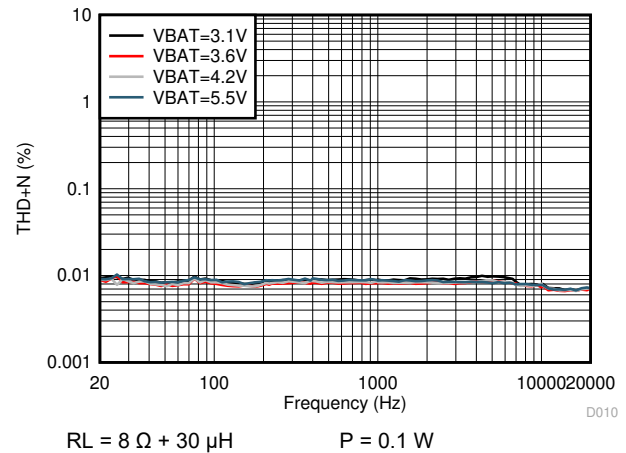
図 5-18. THD+N vs Frequency
