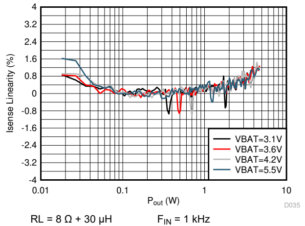
図 5-42. I-sense Linearity vs Output Power
