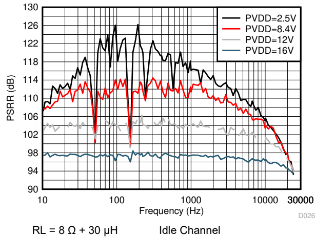
Figure 5-33. PVDD PSRR vs Frequency
