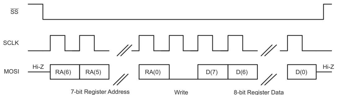
図 7-4. SPI Timing Diagram for Register Write
