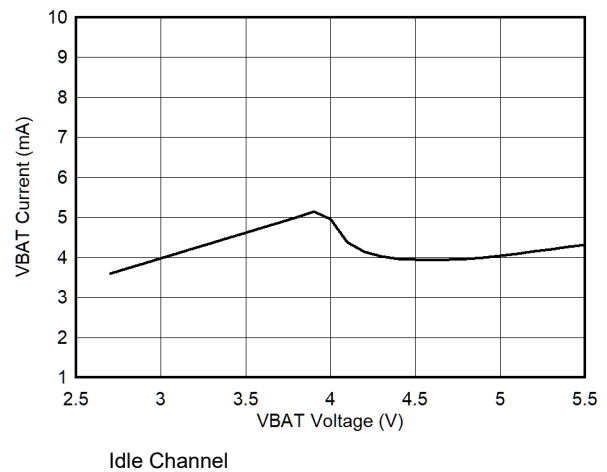
Figure 5-36. VBAT Idle Current vs VBAT
