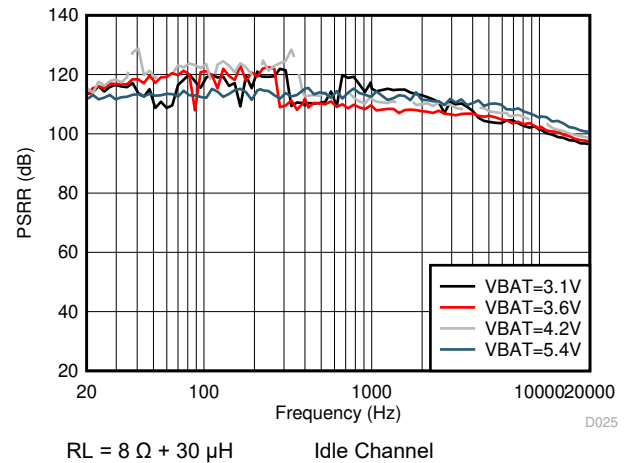
図 5-32. VBAT PSRR vs Frequency
