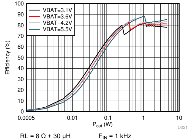
図 5-28. Efficiency vs Output Power
