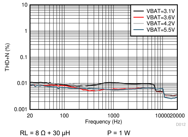
図 5-20. THD+N vs Frequency
