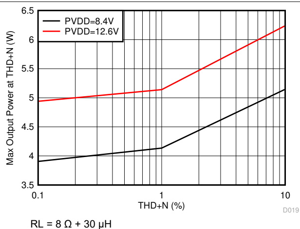
Figure 5-26. Max Output Power vs THD+N
