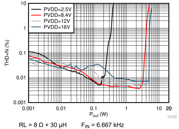
図 5-16. THD+N vs Output Power
