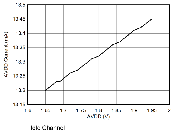
Figure 5-35. AVDD Idle Current vs AVDD (QFN Package)
