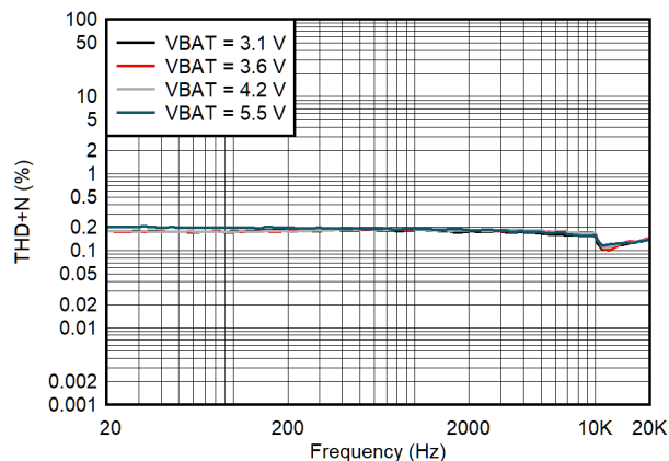
図 5-46. I-sense THD+N vs Frequency (QFN Package)
