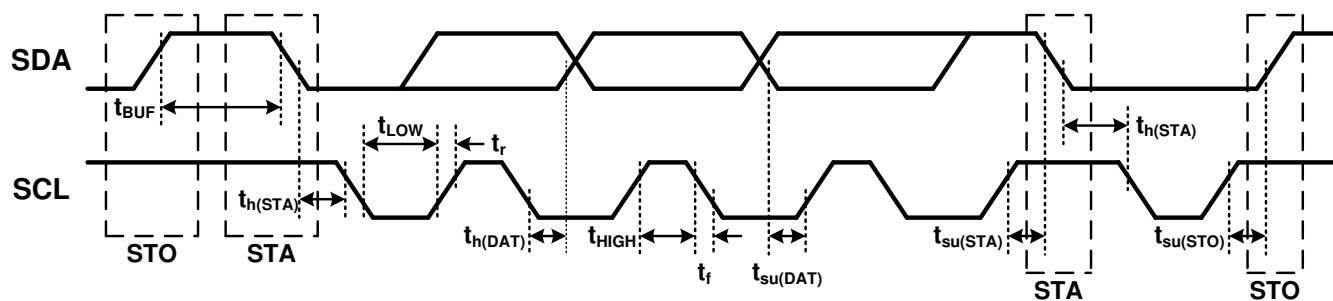
図 5-1. I²C Timing Diagram
