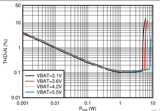
図 5-47. V-sense THD+N vs Output Power
