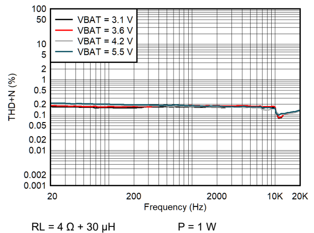
図 5-44. I-sense THD+N vs Frequency (QFN Package)
