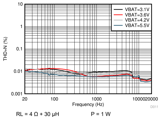
図 5-19. THD+N vs Frequency
