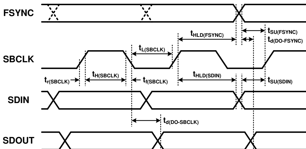
図 5-2. TDM Timing Diagram
