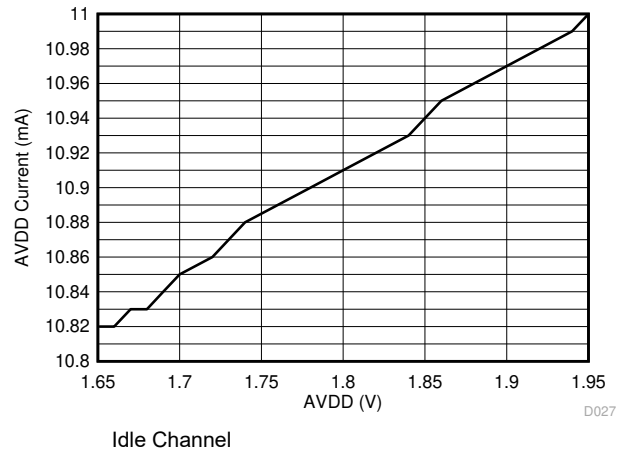
Figure 5-34. AVDD Idle Current vs AVDD (DSBGA Package)
