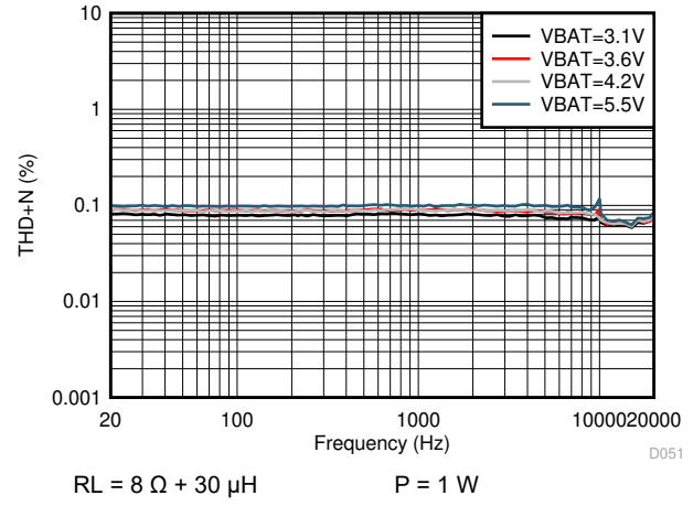
図 5-52. V-sense THD+N vs Frequency
