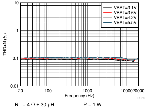
図 5-51. V-sense THD+N vs Frequency
