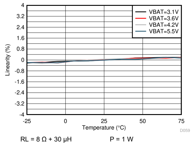
図 5-56. V-sense Linearity vs Temperature
