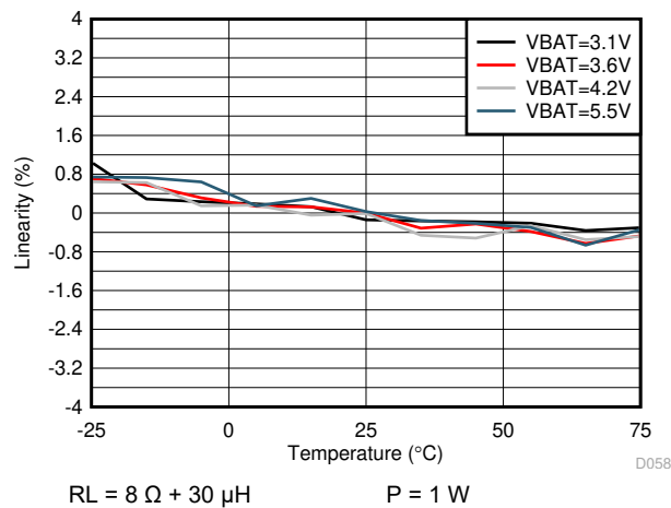
図 5-55. I-sense Linearity vs Temperature
