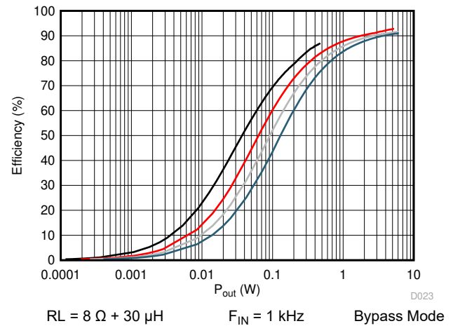
図 5-30. Efficiency vs Output Power
