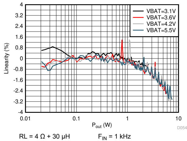
図 5-53. V/I-sense Linearity vs Output Power
