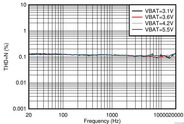
図 5-45. I-sense THD+N vs Frequency (DSBGA Package)
