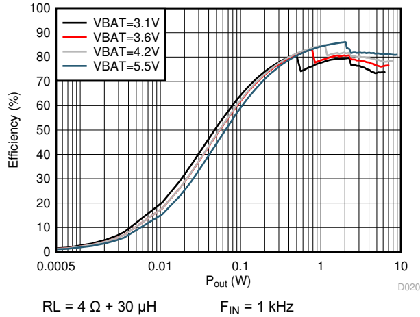
図 5-27. Efficiency vs Output Power
