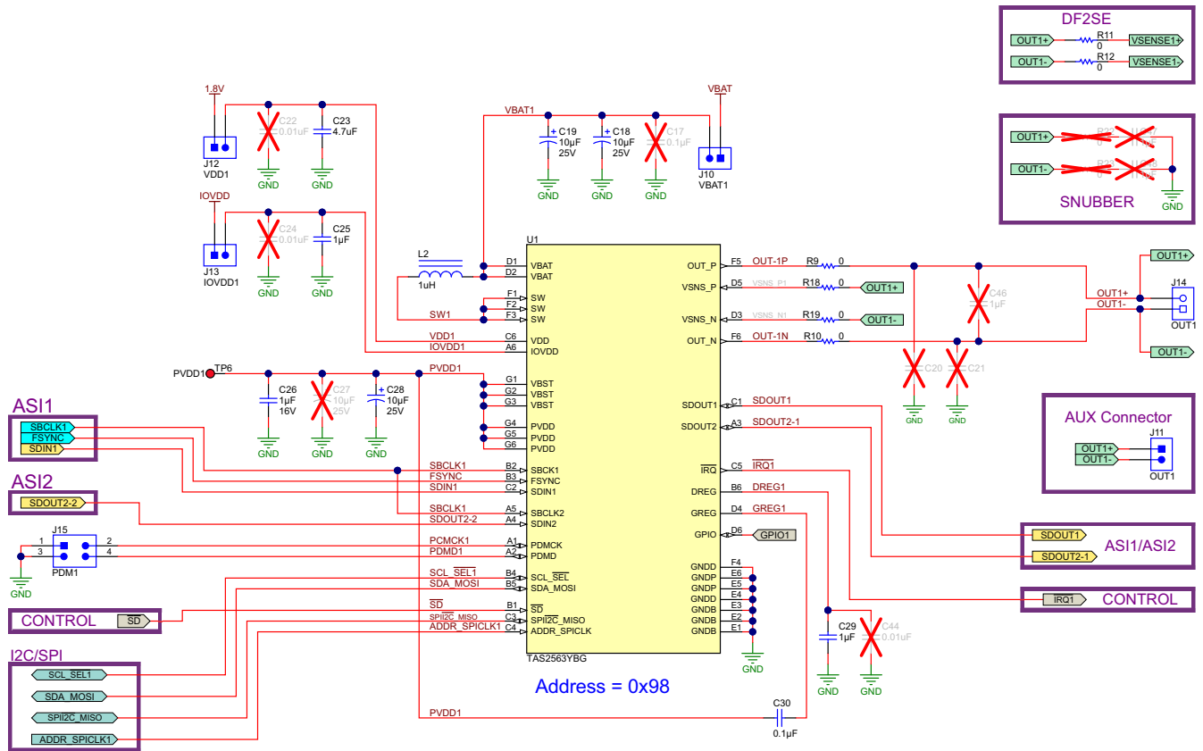
6-1. TAS2563 Circuit
