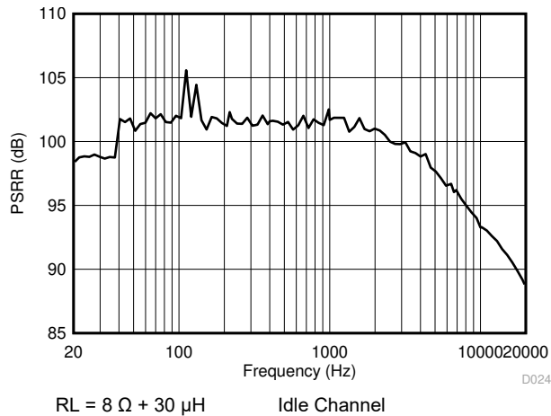
図 5-31. AVDD PSRR vs Frequency
