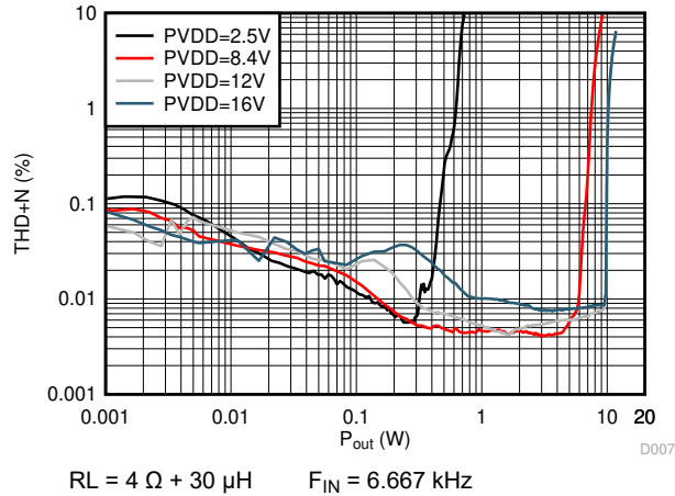
図 5-15. THD+N vs Output Power
