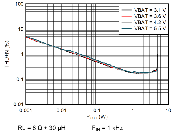
図 5-40. I-sense THD+N vs Output Power (QFN Package)
