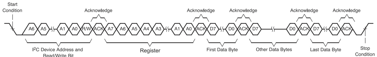
Figure 7-7. Multi-Byte Write Transfer
