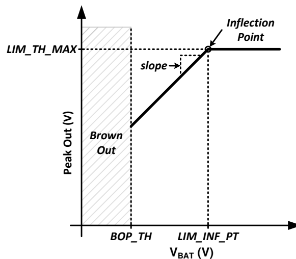
図 7-16. Limiter with Inflection Point
