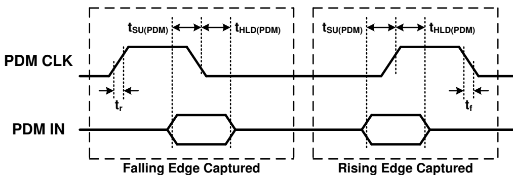
図 5-3. PDM Timing Diagram
