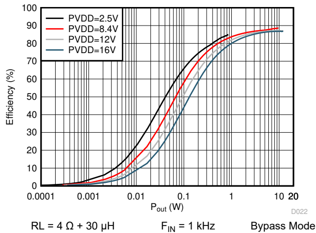
図 5-29. Efficiency vs Output Power
