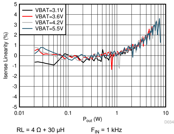
図 5-41. I-sense Linearity vs Output Power
