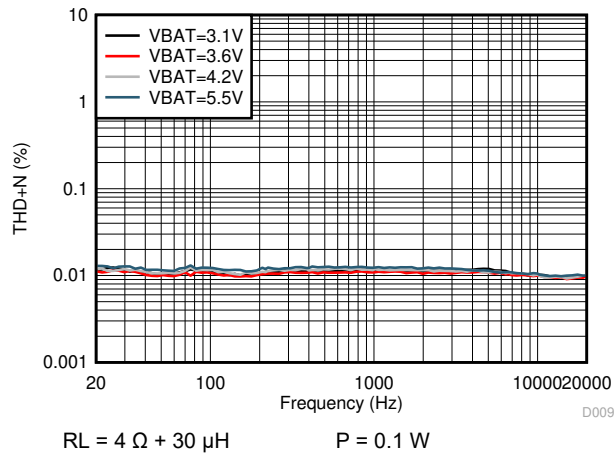
図 5-17. THD+N vs Frequency
