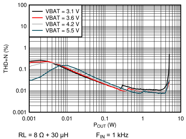
図 5-8. THD+N vs Output Power (QFN Package)
