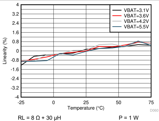
図 5-57. V/I-sense Linearity vs Temperature
