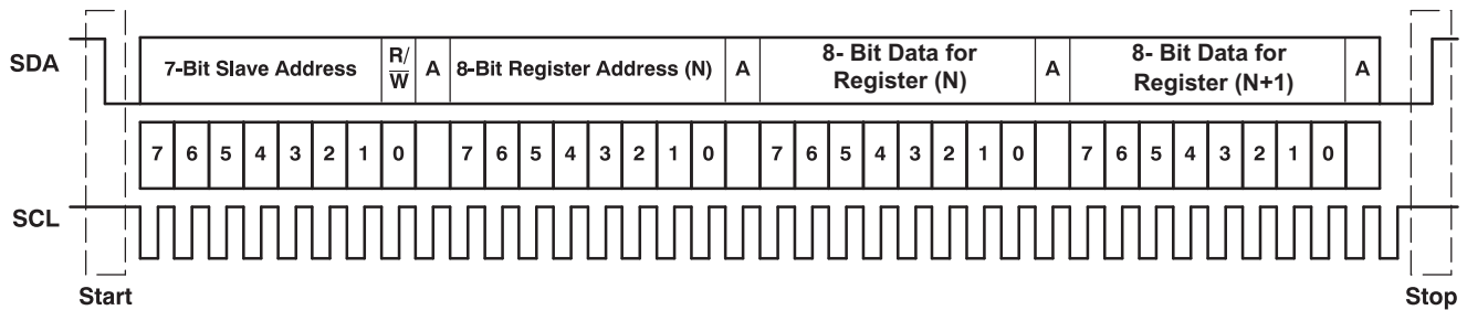
FIG 50. Typical I²C Sequence
