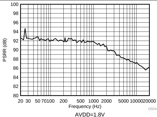
Figure 26. AVDD PSRR vs Frequency
