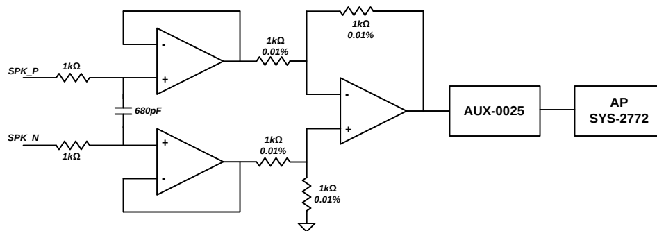
FIG 49. Differential To Single Ended (D2S) Filter
