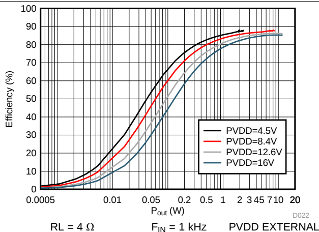
Figure 24. Efficiency vs Output Power
