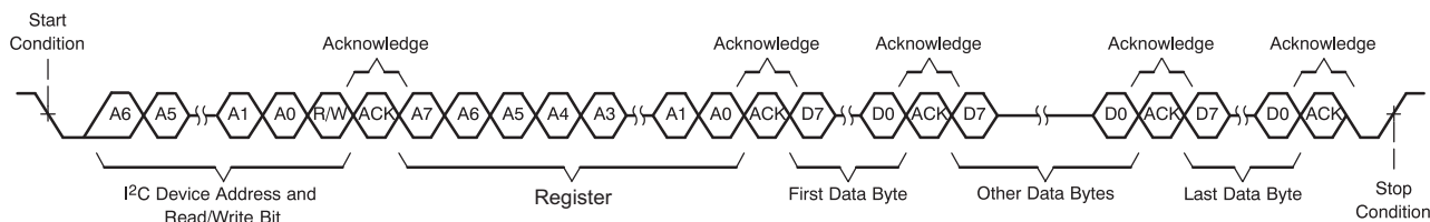
Figure 27. Multiple-Byte Write Transfer
