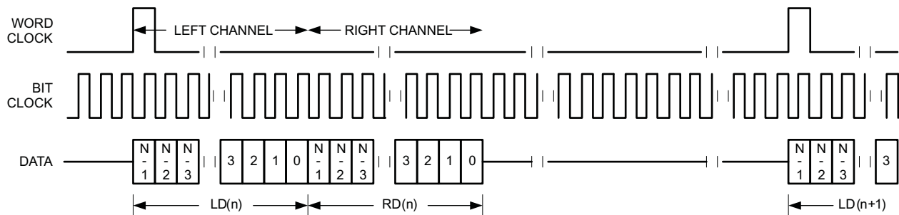
FIG 39. Timing Diagram for DSP Mode with ASI_OFFSET1=0 and Inverted Bit Clock
