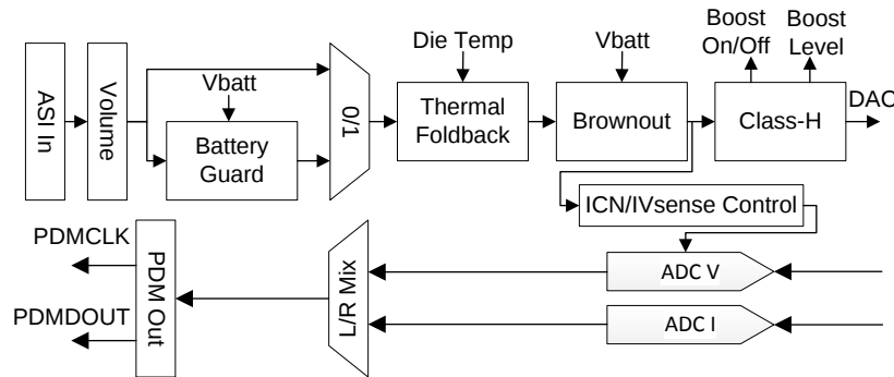
图 54. Mode 3 Processing Block Diagram
