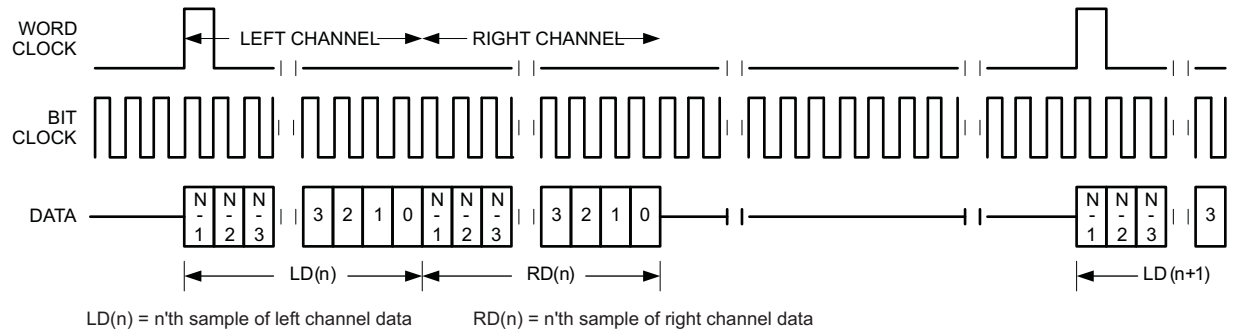
FIG 37. Timing Diagram for DSP Mode
