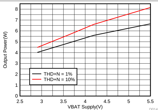
FIG 20. Output Power for 1% and 10% THD+N vs VBAT
