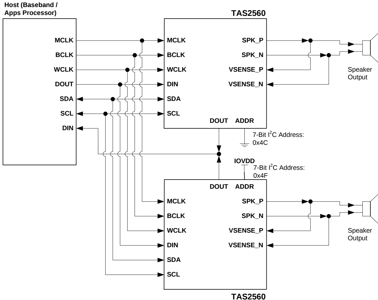
✎ 49. Stereo Configuration with Two TAS2560 DOUT Muxed in TDM Mode
