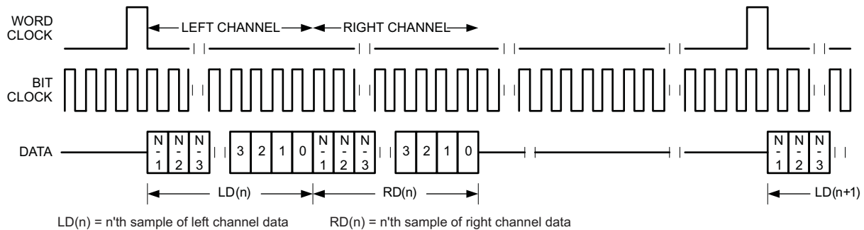
FIG 38. Timing Diagram for DSP Mode with ASI_OFFSET1=1
