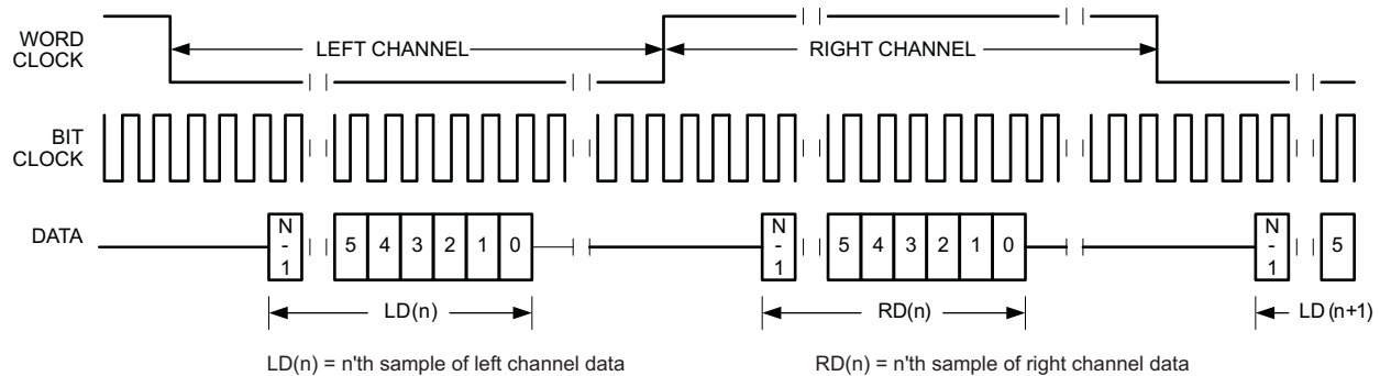
FIG 48. Timing Diagram for I 2 S in TDM Mode with ASI_OFFSET1=2
