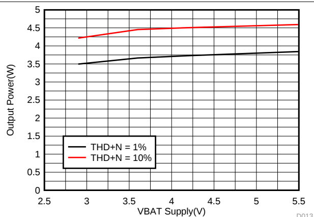
FIG 19. Output Power for 1% and 10% THD+N vs VBAT
