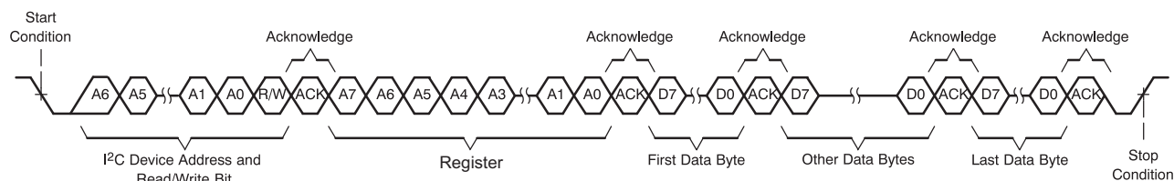
FIG 21. Multiple-Byte Write Transfer
