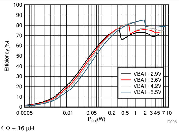
FIG 14. Efficiency vs Output Power
