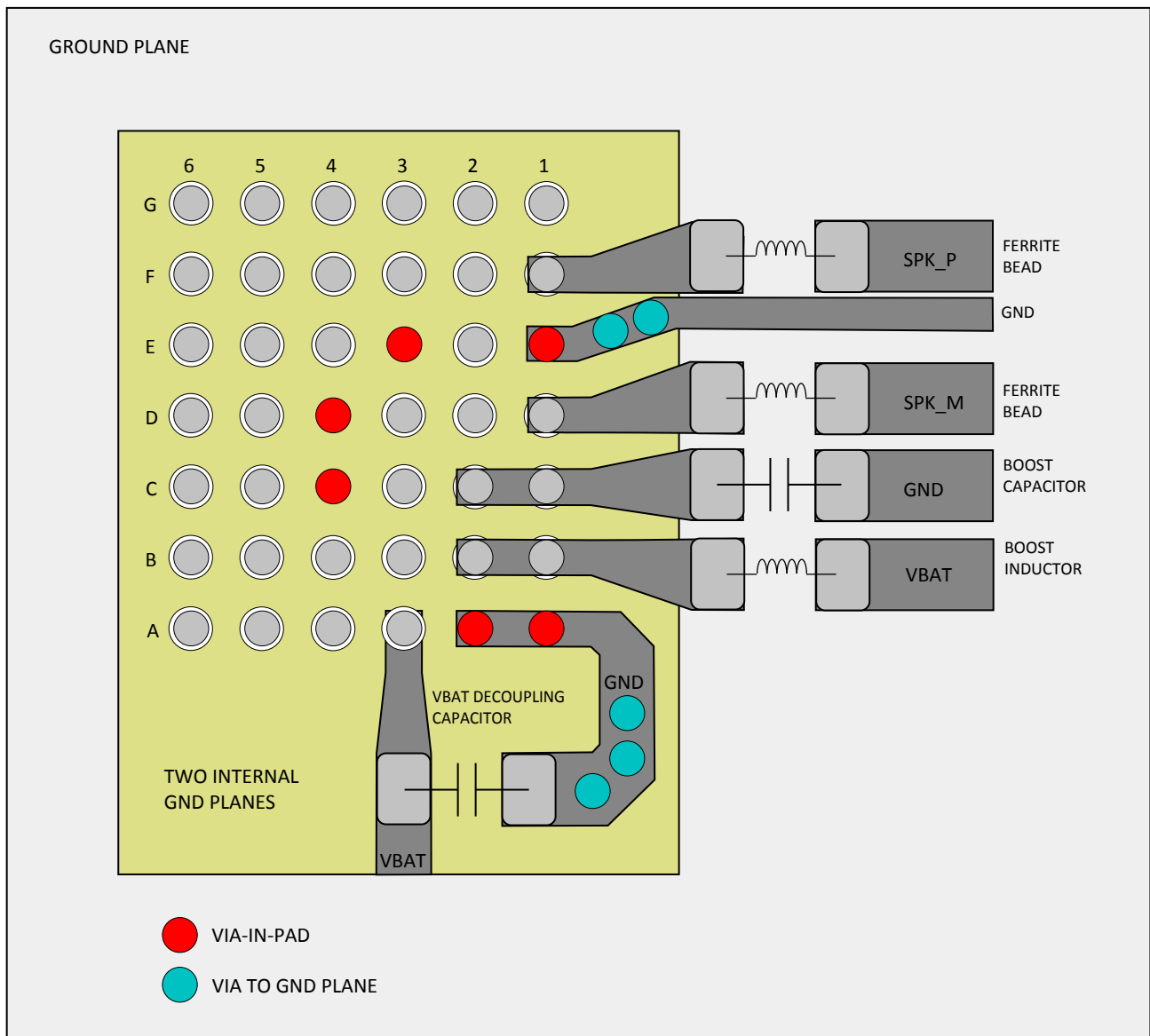
FIG 151. TAS2557 Board Layout
