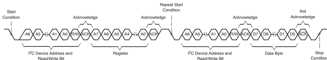
FIG 22. Single-Byte Read Transfer
