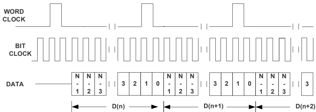
FIG 40. Timing Diagram for Mono PCM Mode with ASI\_OFFSET1=2
