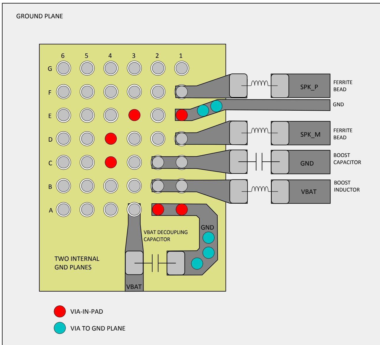
41. TAS2555 Board Layout
