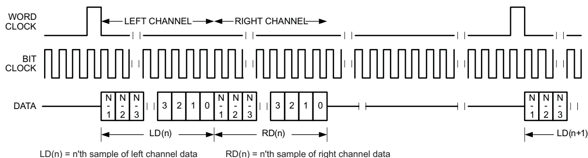
FIG 33. Timing Diagram for DSP Mode with Offset=1
