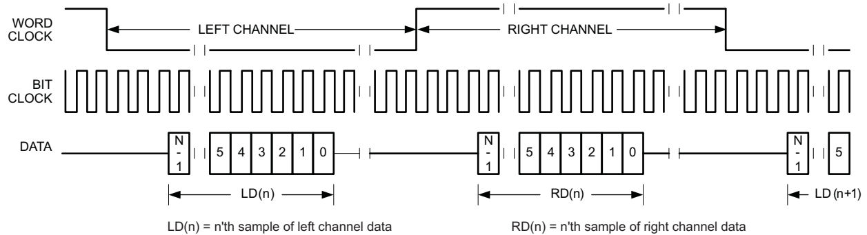
FIG 30. Timing Diagram for I 2 S Mode with Offset = 2
