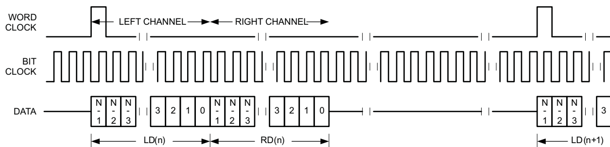
FIG 34. Timing Diagram for DSP Mode with Offset=0 and Inverted Bit Clock
