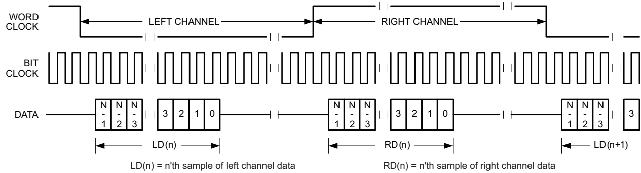
FIG 29. Timing Diagram for I 2 S Mode
