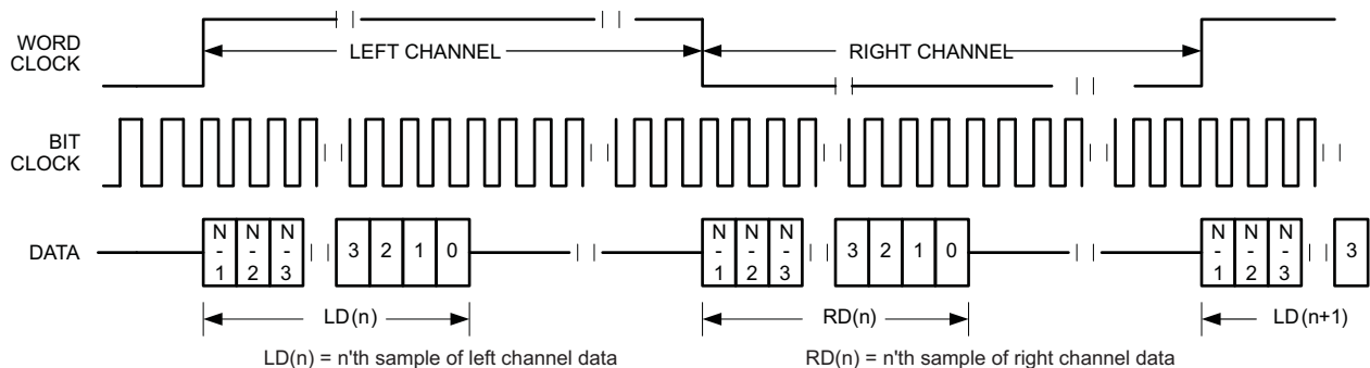
FIG 28. Timing Diagram for Left-Justified Mode with Offset = 0 and Inverted Bit Clock
