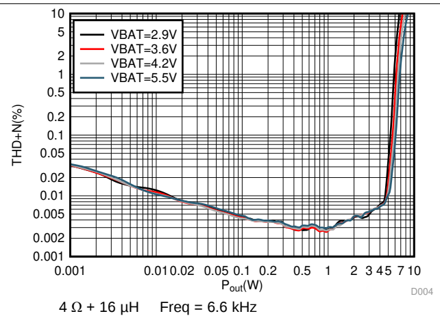
图 10. THD+N vs Output Power
