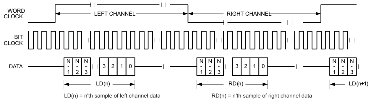
FIG 27. Timing Diagram for Light-Left Mode with Offset = 1
