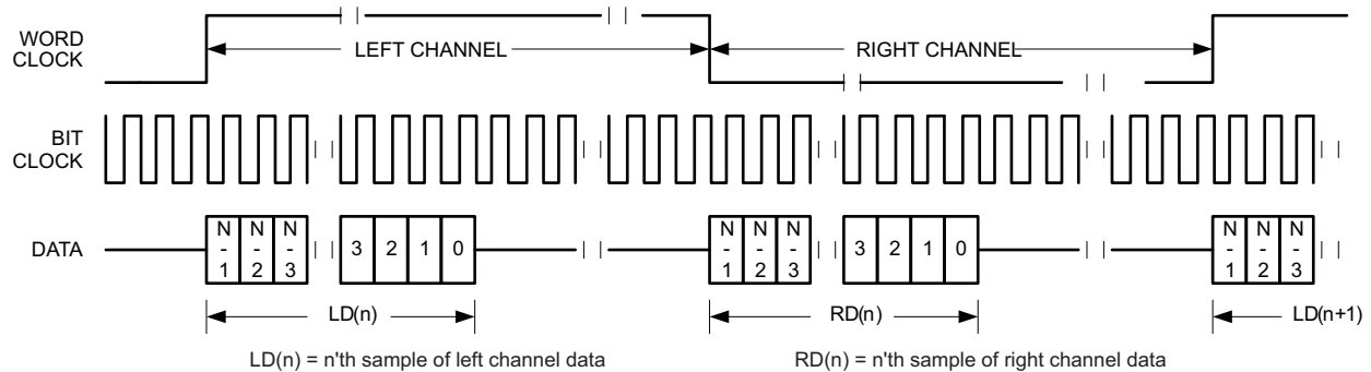
FIG 26. Timing Diagram for Left-Justified Mode
