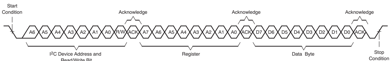
✎ 20. Single-Byte Write Transfer
