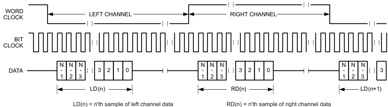
FIG 31. Timing Diagram for I 2 S Mode with Offset = 0 and Inverted Bit Clock
