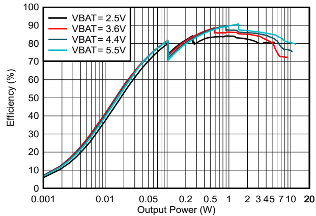
図 7-3. Efficiency vs Output Power
