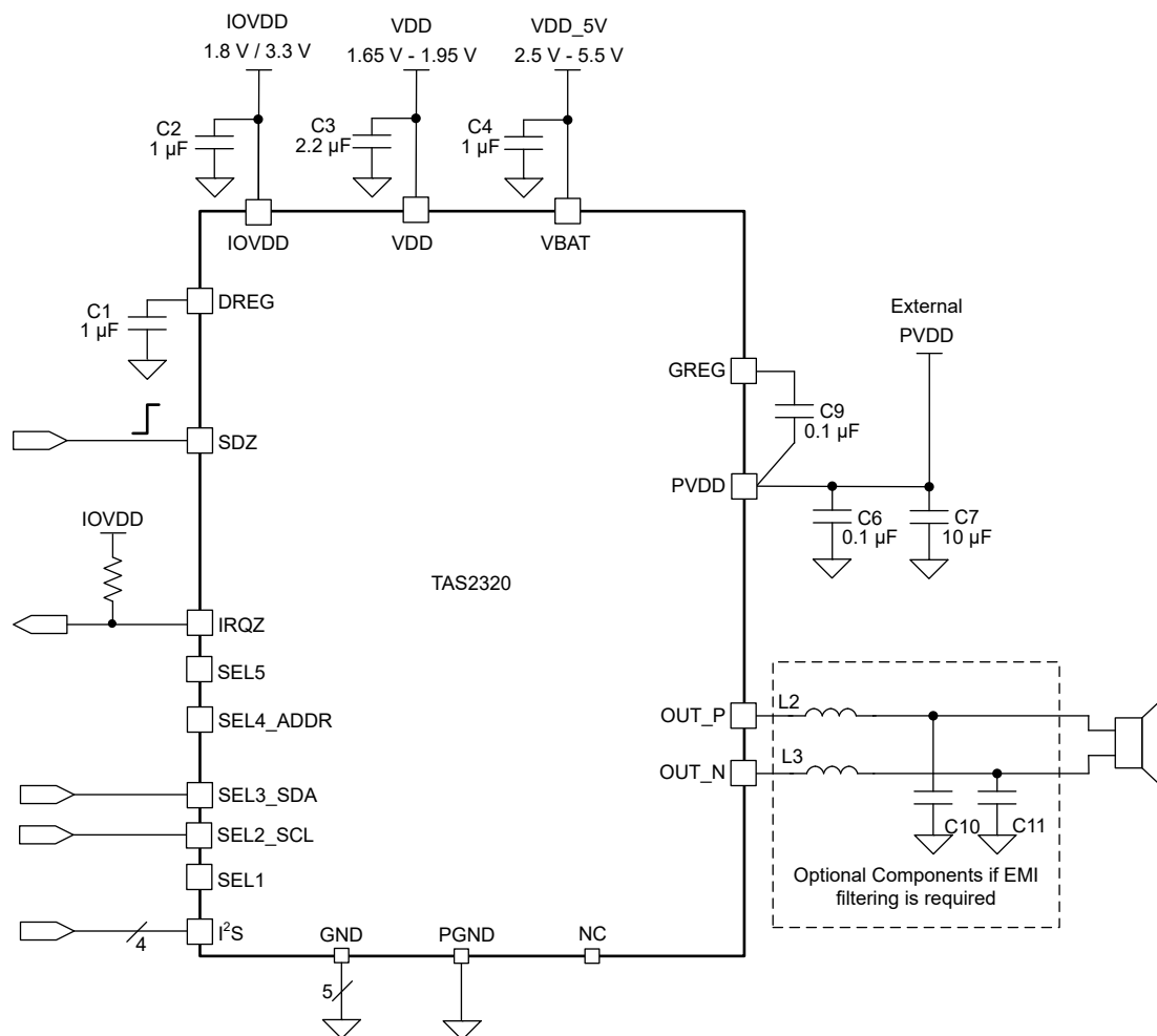
図 7-1. Application Diagram for External PVDD or 3S Battery system
