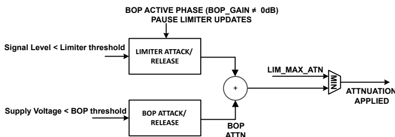
図 6-3. Limiter and Brown out gain attenuation
