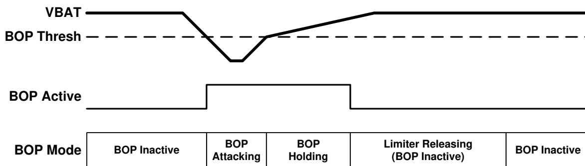
図 6-2. Brown Out Prevention Event
