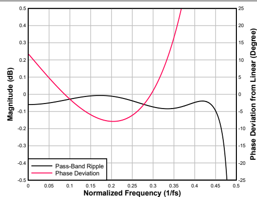
図 6-51. Ultra-Low-Latency interpolation Filter Pass-Band Ripple and Phase Deviation
