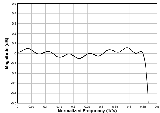
図 6-73. Linear-phase Decimation Filter Pass-Band Ripple
