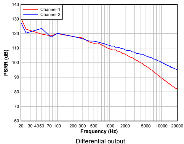
Figure 5-18. DAC PSRR vs Frequency
