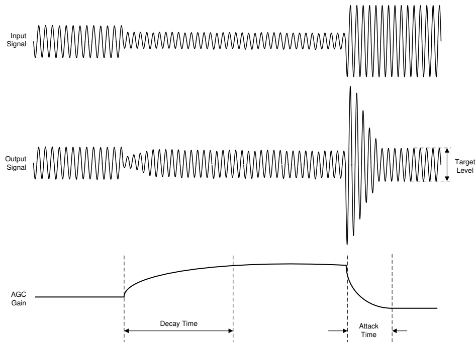
Figure 6-100. AGC Characteristics
