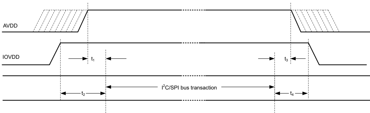
図 8-4. Power-Supply Sequencing Requirement Timing Diagram
