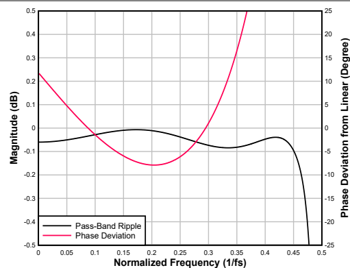
図 6-53. Ultra-Low-Latency interpolation Filter Pass-Band Ripple and Phase Deviation
