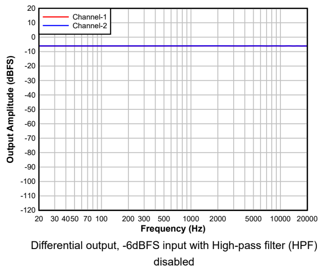
Figure 5-20. DAC Frequency Response
