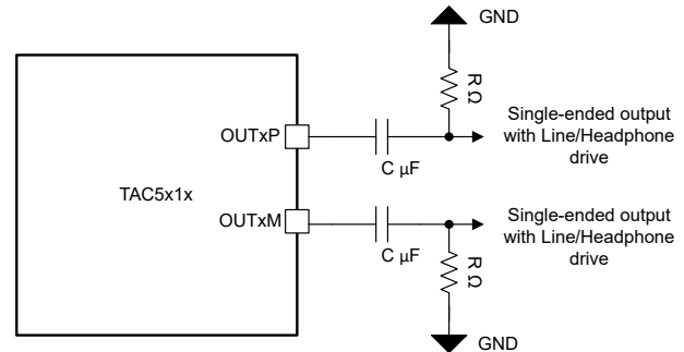
図 6-17. Stereo Single-ended Output Connection (OUT1x_CFG[2:0] = 3'b001)
