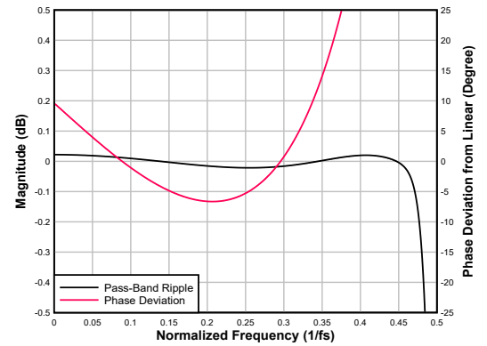
図 6-96. Ultra Low-latency Decimation Filter Pass-Band Ripple and Phase Deviation
