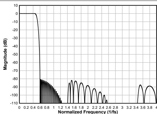
図 6-69. Linear-phase Decimation Filter Magnitude Response
