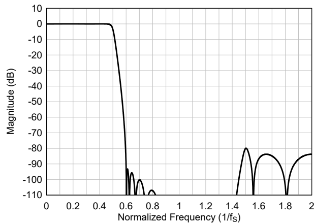
図 6-57. Ultra-Low-Latency interpolation Filter Magnitude Response
