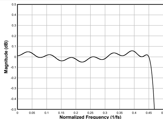
図 6-74. Linear-phase Decimation Filter Pass-Band Ripple
