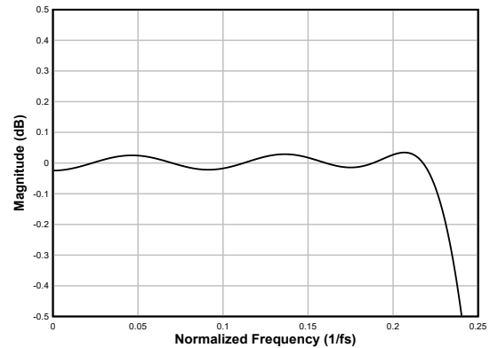
図 6-76. Linear-phase Decimation Filter Pass-Band Ripple
