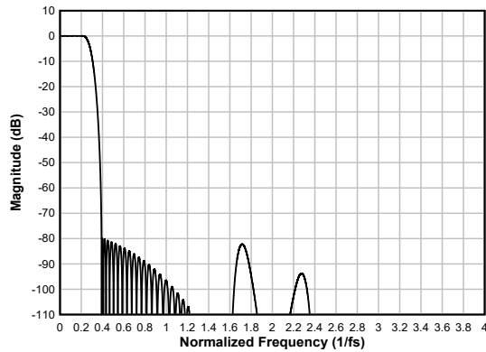
図 6-75. Linear-phase Decimation Filter Magnitude Response
