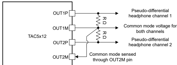
図 6-17. Psuedo-differential Output Connection with External Common-Mode Sense (OUT1x_CFG[2:0] = 3'b101)
