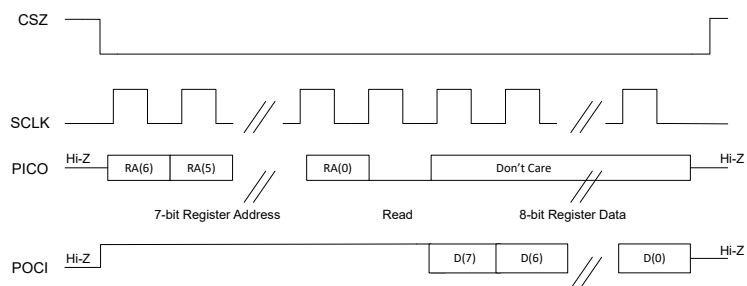
图 6-108. SPI Single-Byte Read Transfer
