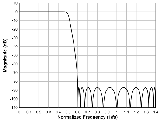
図 6-49. Low-latency Interpolation Filter Magnitude Response
