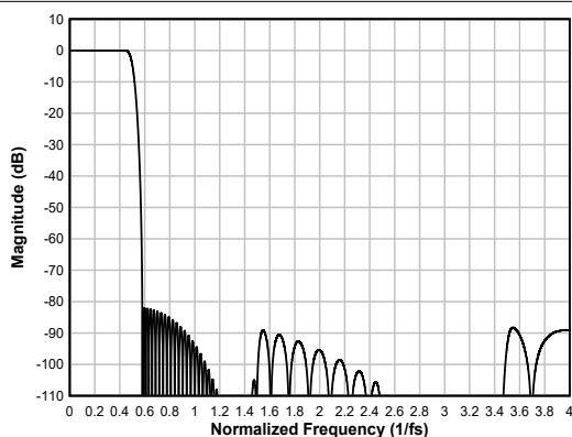
図 6-31. Linear-phase Interpolation Filter Magnitude Response
