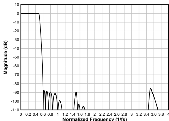
図 6-97. Ultra Low-latency Decimation Filter Magnitude Response
