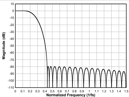
図 6-39. Linear-phase Interpolation Filter Magnitude Response
