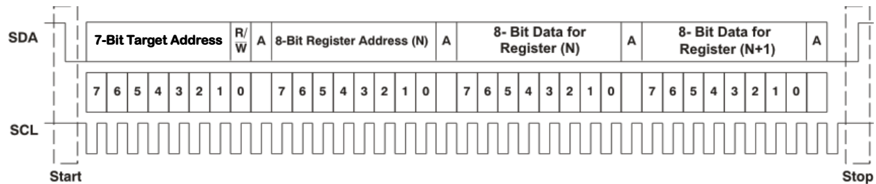
図 6-102. Typical I 2 C Sequence
