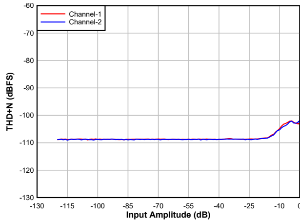
Figure 5-5. DAC THD+N Level vs Input
