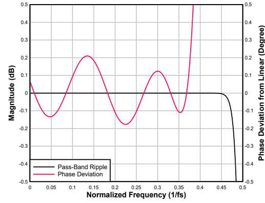
図 6-50. Low-latency Interpolation Filter Pass-Band Ripple and Phase Deviation
