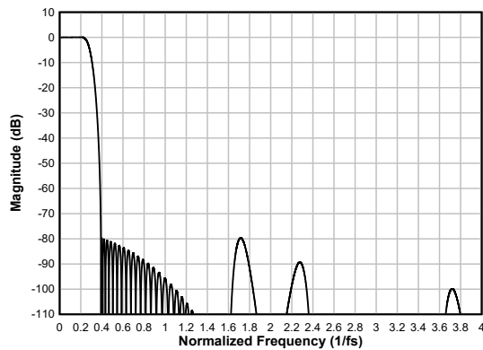
図 6-77. Linear-phase Decimation Filter Magnitude Response
