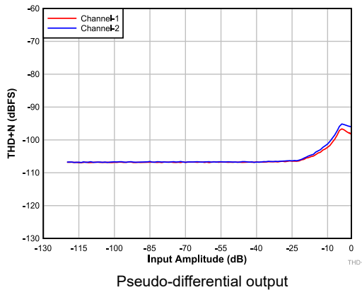
Figure 5-7. DAC THD+N Level vs Input
