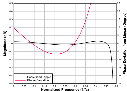
図 6-98. Ultra Low-latency Decimation Filter Pass-Band Ripple and Phase Deviation
