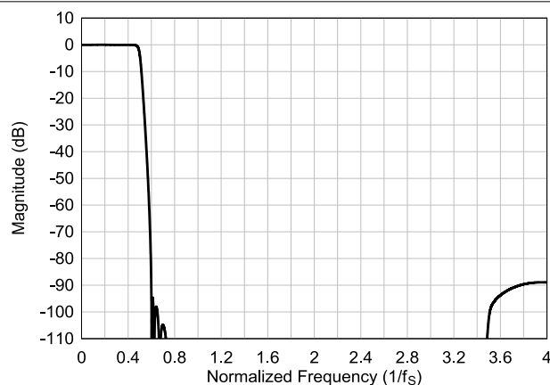
図 6-51. Ultra-Low-Latency interpolation Filter Magnitude Response
