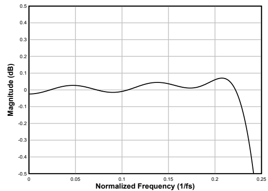
図 6-78. Linear-phase Decimation Filter Pass-Band Ripple
