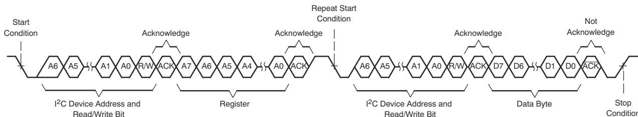
Figure 6-105. I 2 C Single-Byte Read Transfer
