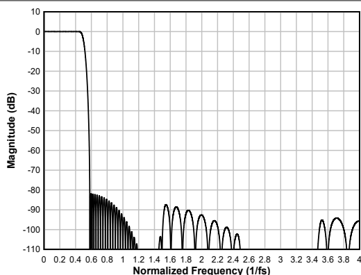
図 6-29. Linear-phase Interpolation Filter Magnitude Response
