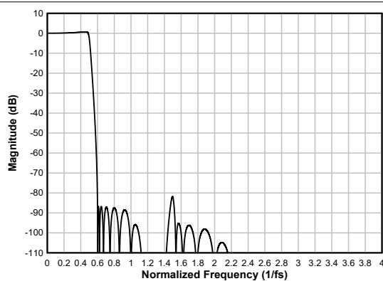
図 6-91. Ultra Low-latency Decimation Filter Magnitude Response
