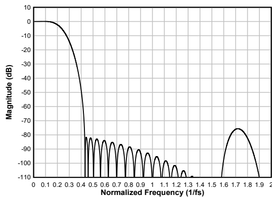
図 6-79. Linear-phase Decimation Filter Magnitude Response
