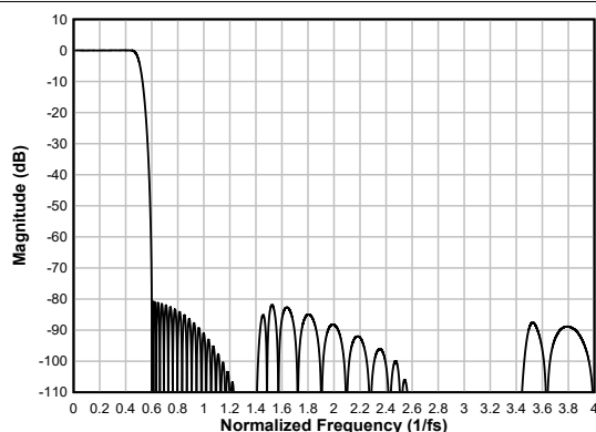
図 6-67. Linear-phase Decimation Filter Magnitude Response
