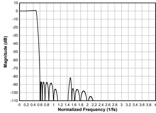
図 6-93. Ultra Low-latency Decimation Filter Magnitude Response
