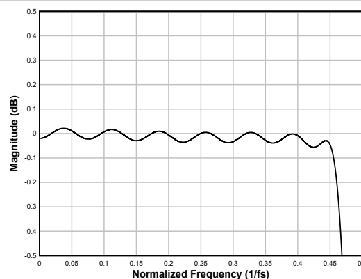
図 6-32. Linear-phase Interpolation Filter Pass-Band Ripple
