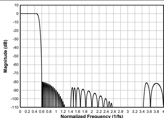
図 6-65. Linear-phase Decimation Filter Magnitude Response
