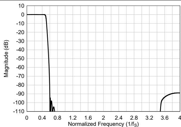
図 6-53. Ultra-Low-Latency interpolation Filter Magnitude Response
