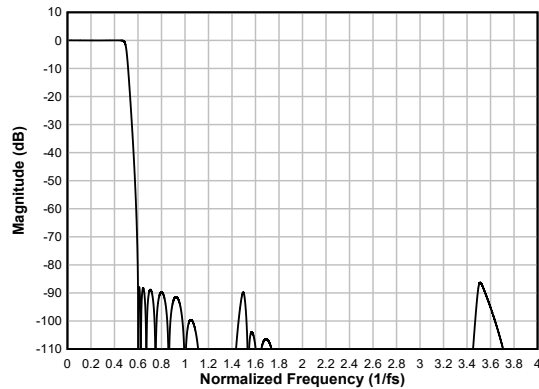
図 6-95. Ultra Low-latency Decimation Filter Magnitude Response
