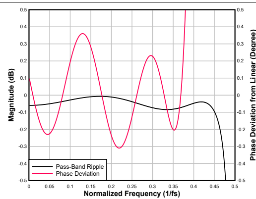
図 6-42. Low-latency Interpolation Filter Pass-Band Ripple and Phase Deviation
