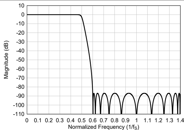
図 6-59. Ultra-Low-Latency interpolation Filter Magnitude Response
