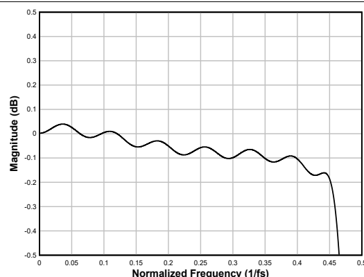
図 6-34. Linear-phase Interpolation Filter Pass-Band Ripple
