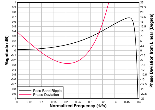
図 6-94. Ultra Low-latency Decimation Filter Pass-Band Ripple and Phase Deviation
