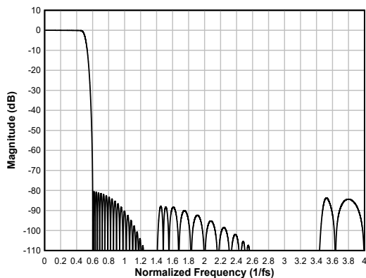
図 6-23. Linear-phase Interpolation Filter Magnitude Response
