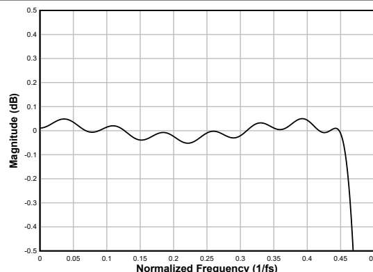
図 6-72. Linear-phase Decimation Filter Pass-Band Ripple
