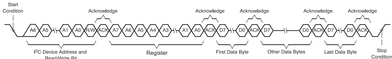
Figure 6-104. I 2 C Multiple-Byte Write Transfer
