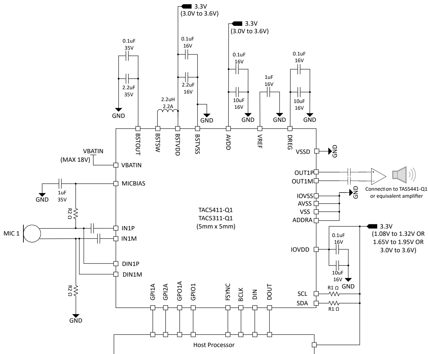
図 8-1. Mono Microphone with Mono Lineout Block Diagram
