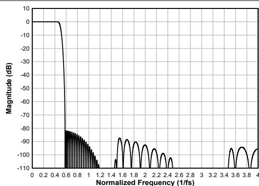
図 6-40. Linear Phase Interpolation Filter Magnitude Response
