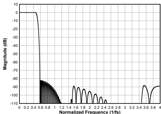
図 6-42. Linear Phase Interpolation Filter Magnitude Response
