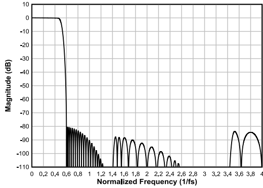
図 6-36. Linear Phase Interpolation Filter Magnitude Response
