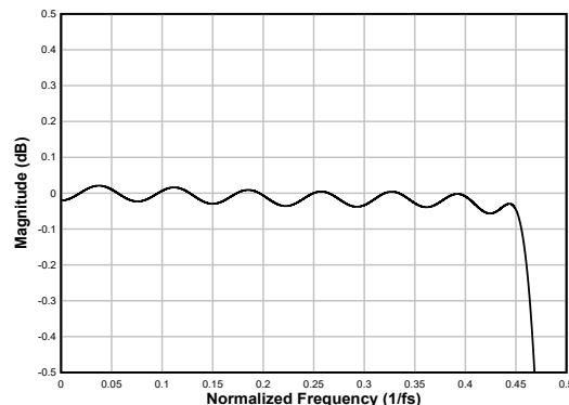
図 6-43. Linear Phase Interpolation Filter Pass-Band Ripple
