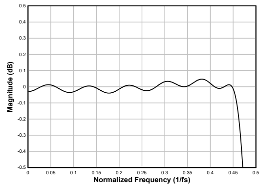
図 6-27. Linear Phase Decimation Filter Pass-Band Ripple
