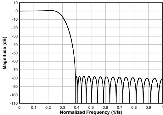
図 6-46. Linear Phase Interpolation Filter Magnitude Response
