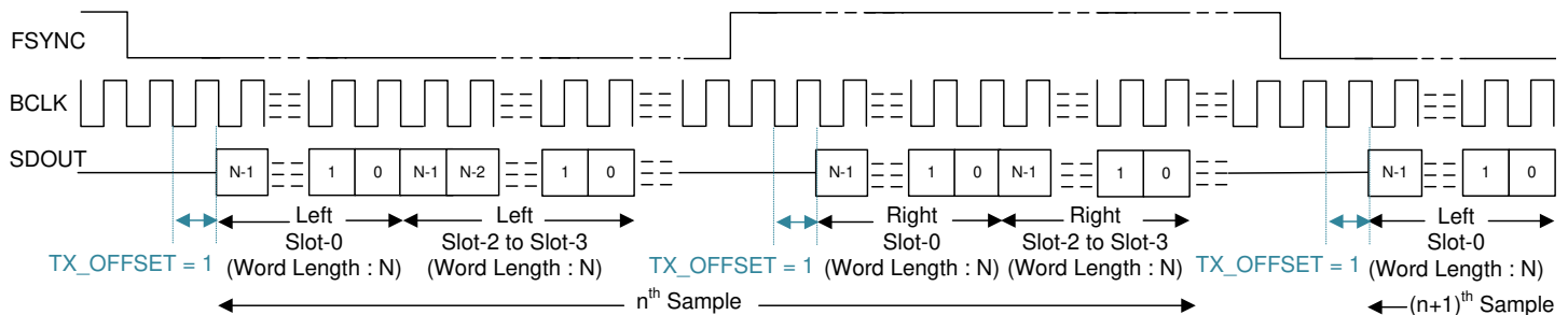
図 6-7. I 2 S Protocol Timing (PASI_TX_OFFSET = 1)
