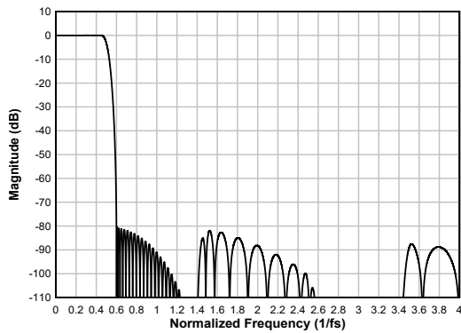
図 6-26. Linear Phase Decimation Filter Magnitude Response
