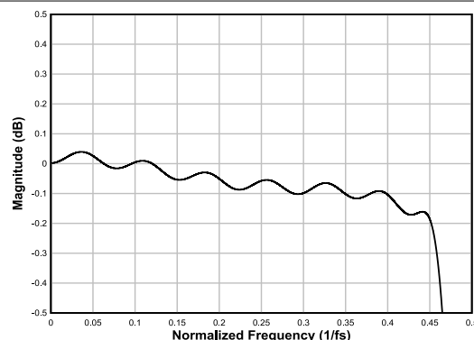
図 6-45. Linear Phase Interpolation Filter Pass-Band Ripple
