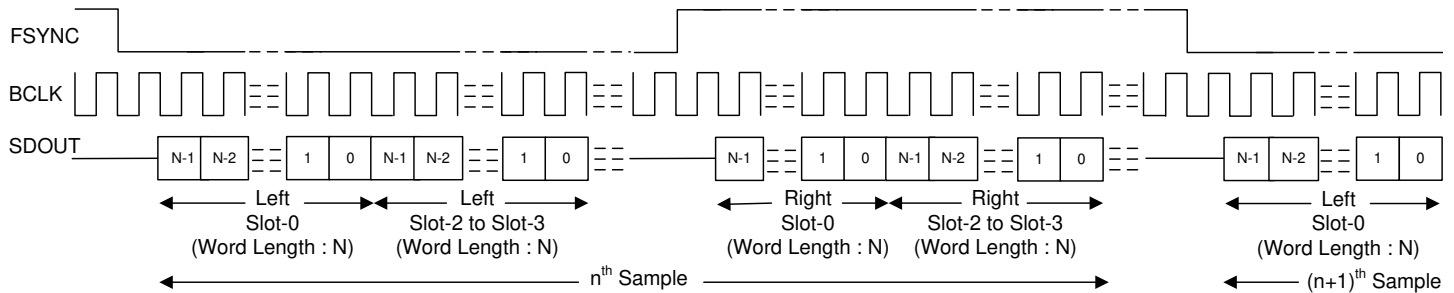
図 6-6. I 2 S Mode Standard Protocol Timing (PASI_TX_OFFSET = 0)
