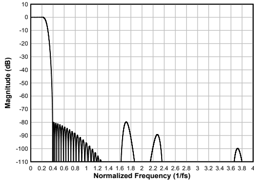
図 6-32. Linear Phase Decimation Filter Magnitude Response
