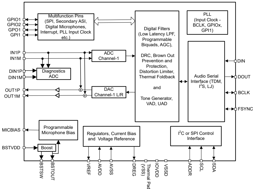
图 6-1. Functional Block Diagram
