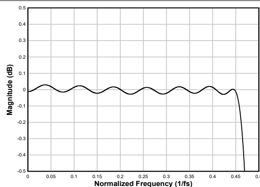
図 6-41. Linear Phase Interpolation Filter Pass-Band Ripple
