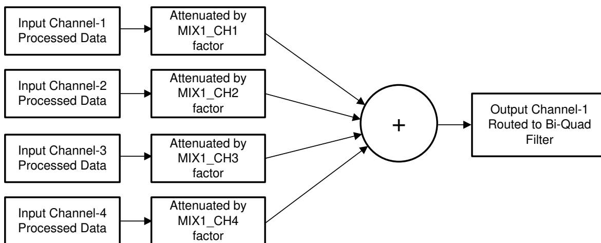
図 6-21. Programmable Digital Mixer Block Diagram
