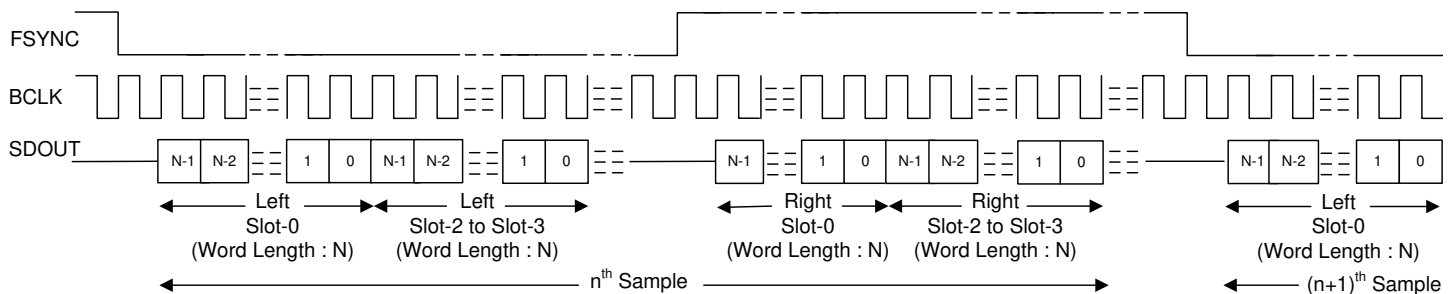
図 6-9. I 2 S Protocol Timing (PASI_TX_OFFSET = 0 and PASI_BCLK_POL = 1)
