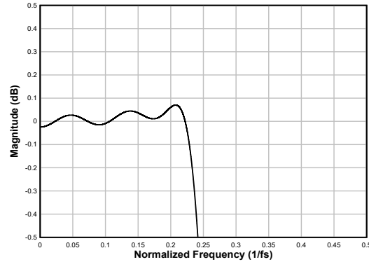
図 6-33. Linear Phase Decimation Filter Pass-Band Ripple
