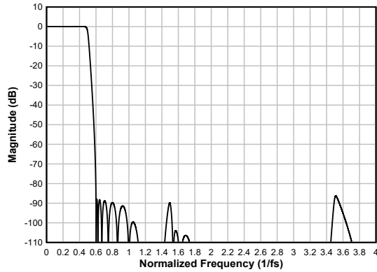
図 6-56. Ultra Low-latency Decimation Filter Magnitude Response
