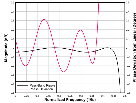
図 6-85. Low-latency Interpolation Filter Pass-Band Ripple and Phase Deviation
