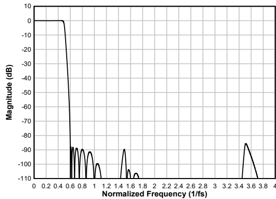
図 6-58. Ultra Low-latency Decimation Filter Magnitude Response
