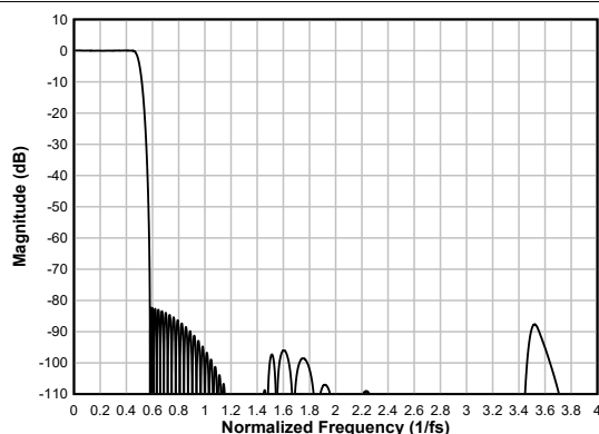
図 6-32. Linear-phase Decimation Filter Magnitude Response
