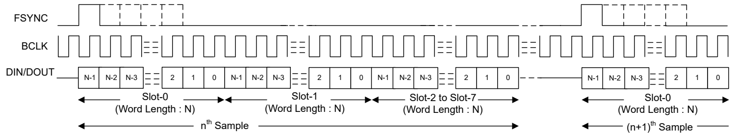
図 6-5. TDM Mode Protocol Timing (PASI_TX_OFFSET = 0 and PASI_BCLK_POL = 1)
