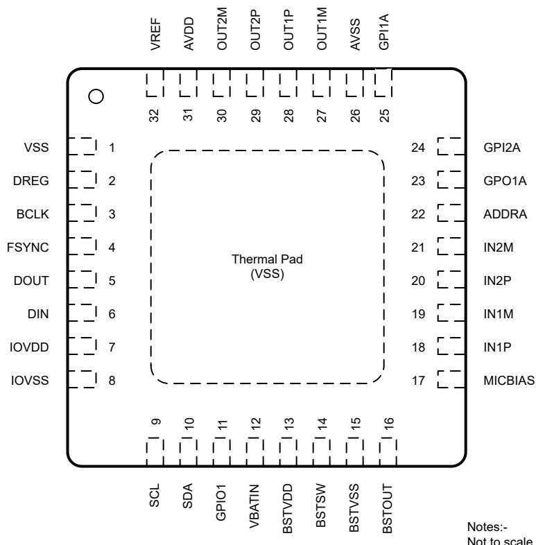
図 4-1. TAC5311-Q1 RTV Package, 32-Pin WQFN With Exposed Thermal Pad, Top View
