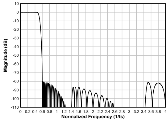
図 6-26. Linear-phase Decimation Filter Magnitude Response
