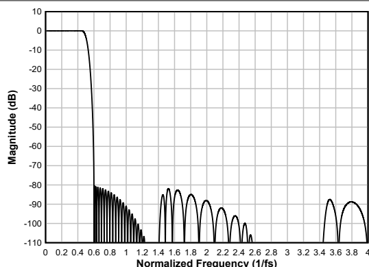
図 6-30. Linear-phase Decimation Filter Magnitude Response
