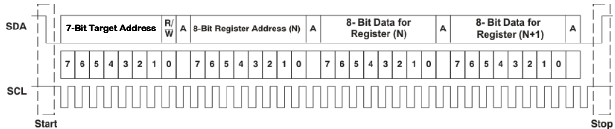
Figure 6-88. Typical I²C Sequence
