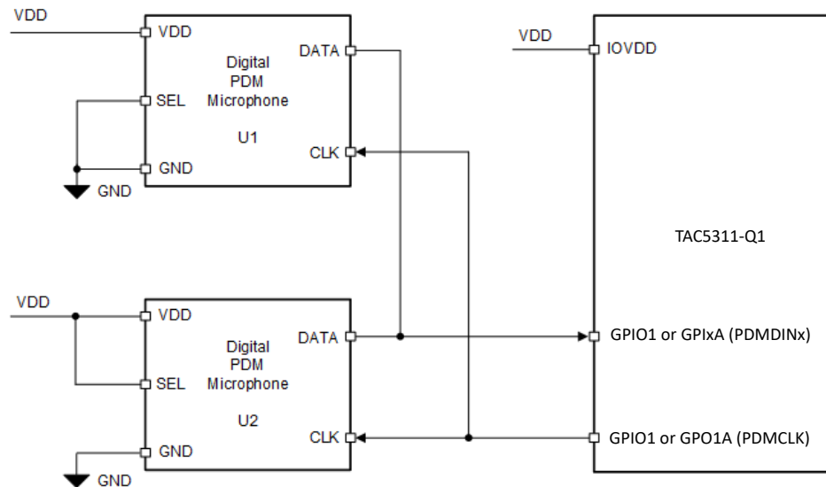
図 6-19. Digital PDM Microphones Connection Diagram for the TAC5311-Q1
