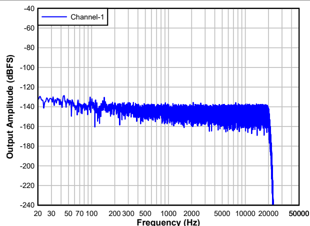
図 5-12. ADC FFT with Idle Channel Input
