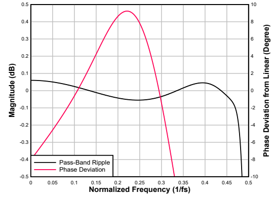
図 6-51. Low-latency Decimation Filter Pass-Band Ripple and Phase Deviation
