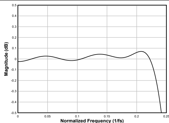
図 6-39. Linear-phase Decimation Filter Pass-Band Ripple
