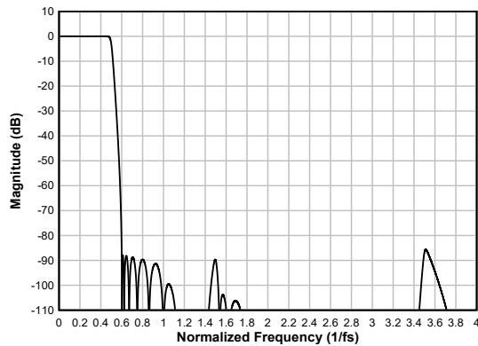
図 6-48. Low-latency Decimation Filter Magnitude Response
