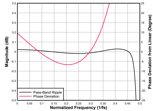
図 6-59. Ultra Low-latency Decimation Filter Pass-Band Ripple and Phase Deviation
