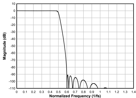
図 6-60. Ultra Low-latency Decimation Filter Magnitude Response
