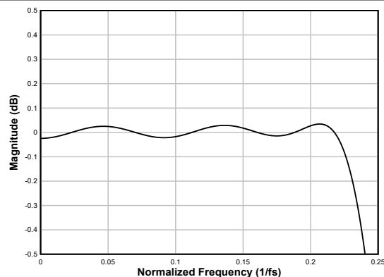
図 6-37. Linear-phase Decimation Filter Pass-Band Ripple
