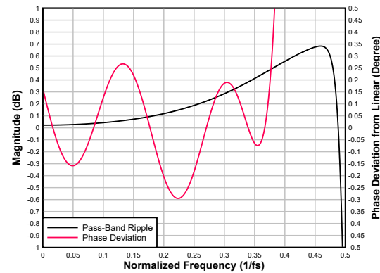
図 6-43. Low-latency Decimation Filter Pass-Band Ripple and Phase Deviation
