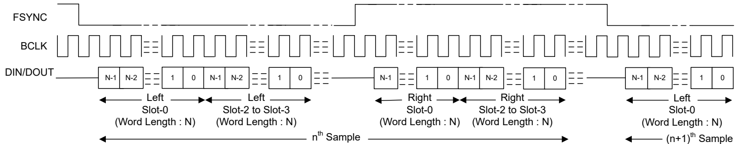
図 6-6. I 2 S Mode Standard Protocol Timing (PASI_TX_OFFSET = 0)
