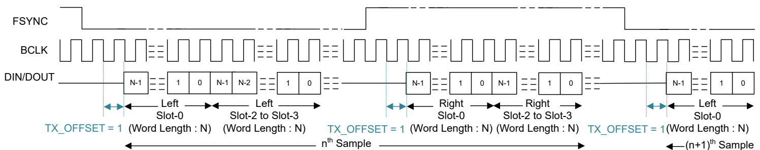
図 6-7. I 2 S Protocol Timing (PASI_TX_OFFSET = 1)
