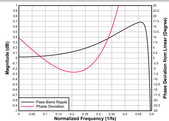
図 6-55. Ultra Low-latency Decimation Filter Pass-Band Ripple and Phase Deviation
