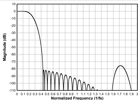
図 6-40. Linear-phase Decimation Filter Magnitude Response
