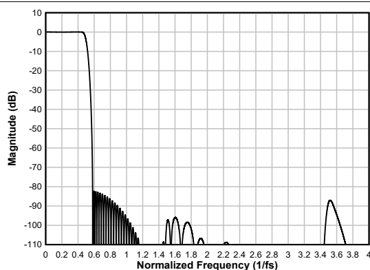
図 6-34. Linear-phase Decimation Filter Magnitude Response
