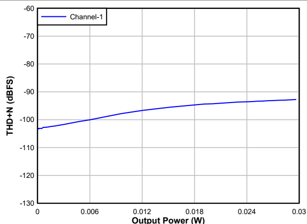
Pseudo-differential headphone output, 16Ω load
