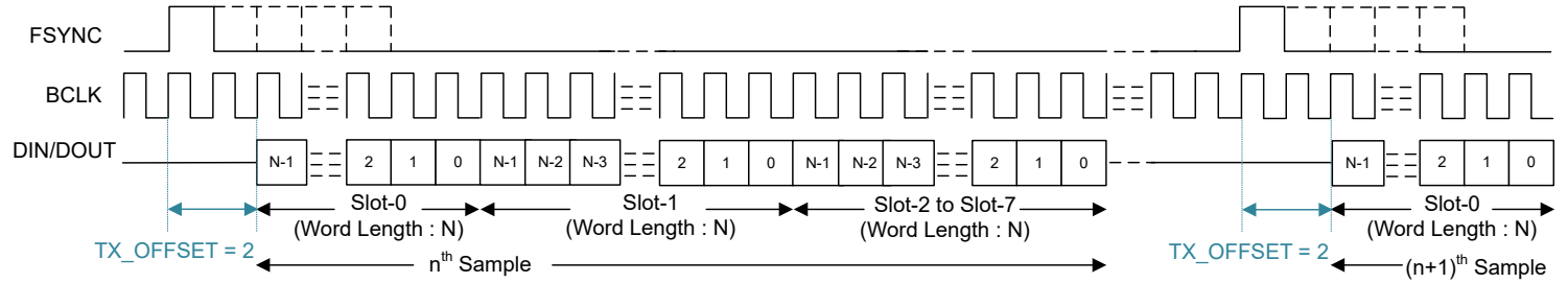
図 6-3. TDM Mode Protocol Timing (PASI_TX_OFFSET = 2)
