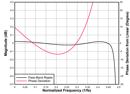
図 6-57. Ultra Low-latency Decimation Filter Pass-Band Ripple and Phase Deviation
