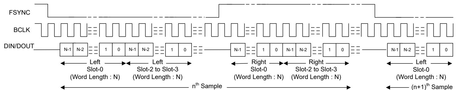
図 6-9. I 2 S Protocol Timing (PASI_TX_OFFSET = 0 and PASI_BCLK_POL = 1)
