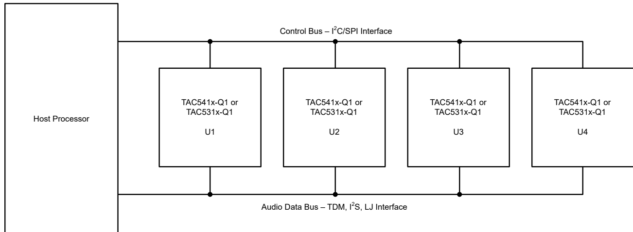
図 6-14. Multiple TAC5311-Q1 Devices With Shared Control and Audio Data Buses
