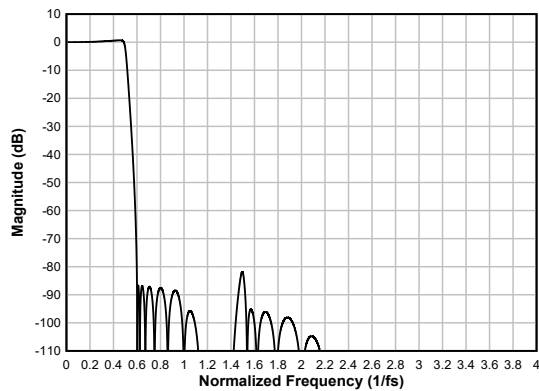
図 6-52. Ultra Low-latency Decimation Filter Magnitude Response
