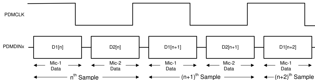
図 6-20. Digital PDM Microphone Protocol Timing Diagram
