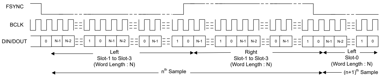
図 6-8. I 2 S Protocol Timing (No Idle BCLK Cycles, PASI_TX_OFFSET = 0)
