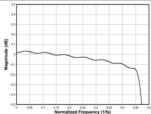
図 6-65. Linear-phase Interpolation Filter Pass-Band Ripple
