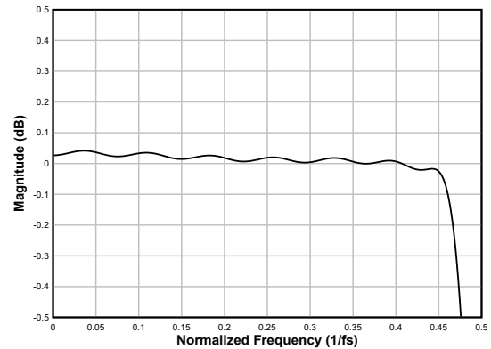
図 6-27. Linear-phase Decimation Filter Pass-Band Ripple
