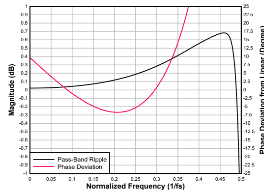
図 6-53. Ultra Low-latency Decimation Filter Pass-Band Ripple and Phase Deviation
