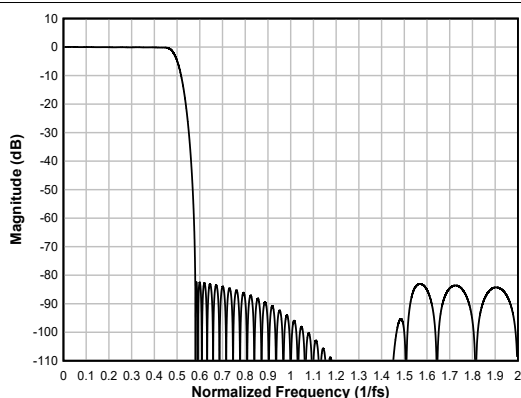
図 6-74. Linear-phase Interpolation Filter Magnitude Response
