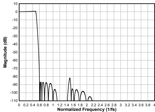
図 6-42. Low-latency Decimation Filter Magnitude Response
