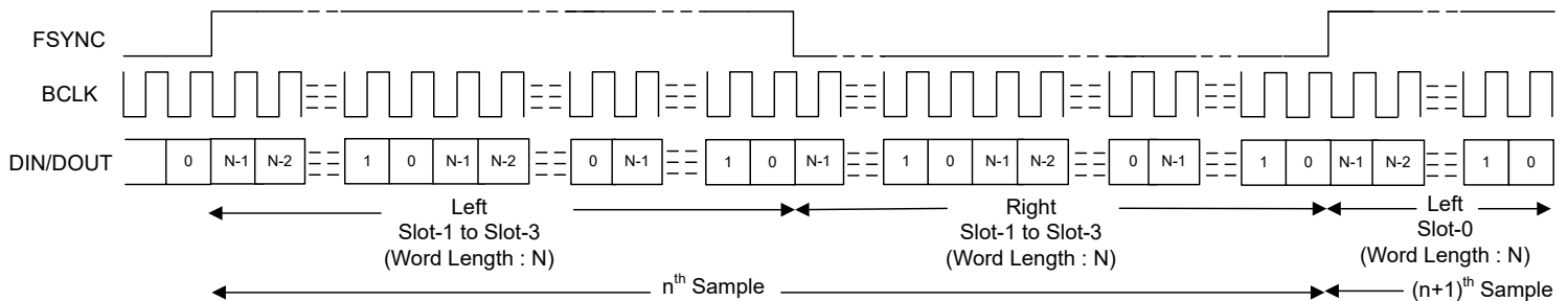
図 6-12. LJ Protocol Timing (No Idle BCLK Cycles, TX_OFFSET = 0)
