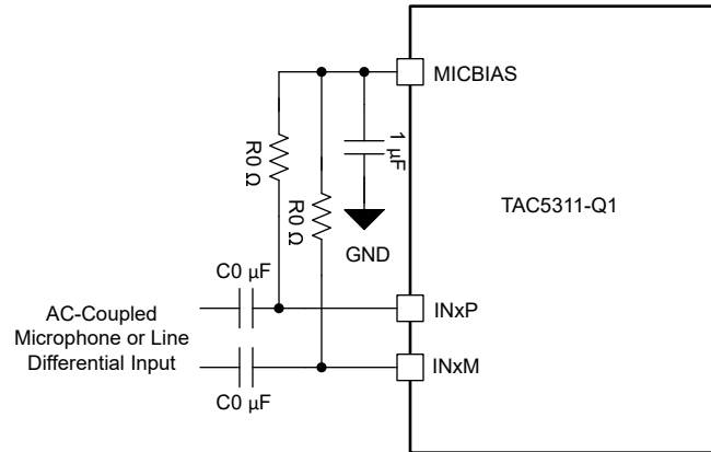
図 6-17. AC-Coupled Microphone or Line Differential Input Connection
