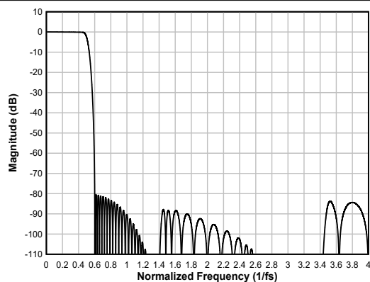
図 6-64. Linear-phase Interpolation Filter Magnitude Response
