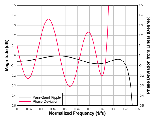
図 6-79. Low-latency Interpolation Filter Pass-Band Ripple and Phase Deviation
