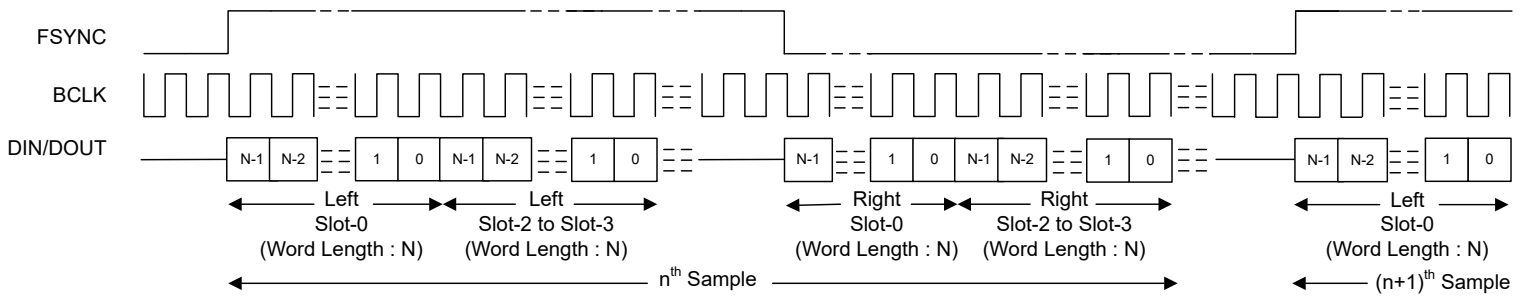
図 6-10. LJ Mode Standard Protocol Timing (TX_OFFSET = 0)
