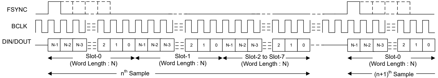
図 6-2. TDM Mode Standard Protocol Timing (PASI_TX_OFFSET = 0)
