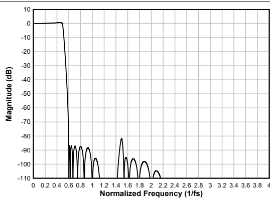
図 6-54. Ultra Low-latency Decimation Filter Magnitude Response
