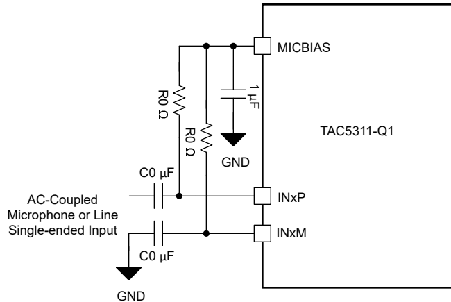
図 6-18. AC-Coupled Microphone or Line Single-Ended Input Connection
