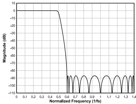
図 6-86. Low-latency Interpolation Filter Magnitude Response
