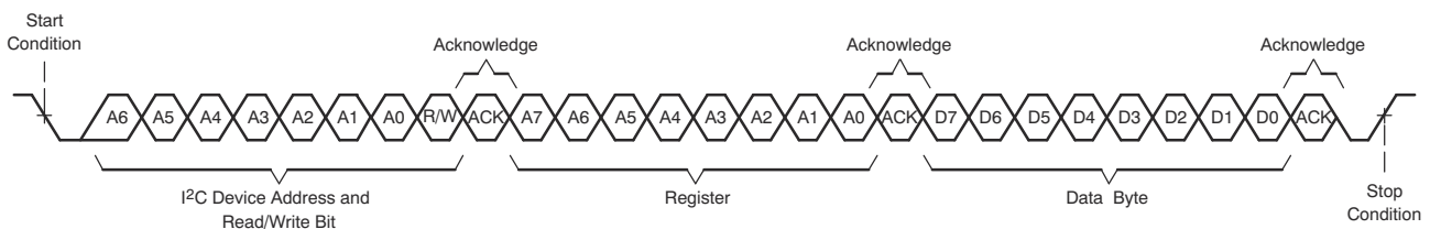
Figure 6-89. I²C Single-Byte Write Transfer
