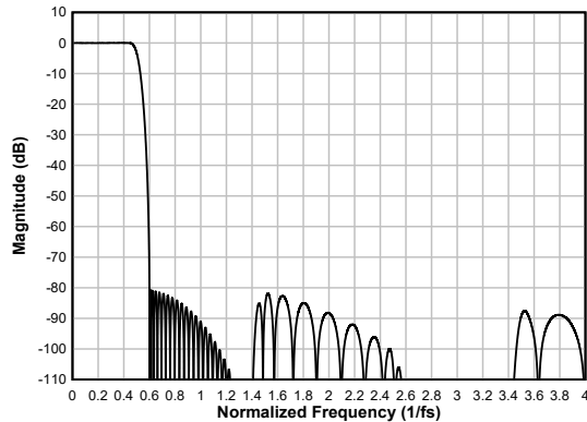
図 6-28. Linear-phase Decimation Filter Magnitude Response
