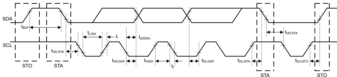
图 5-1. I²C Interface Timing Diagram
