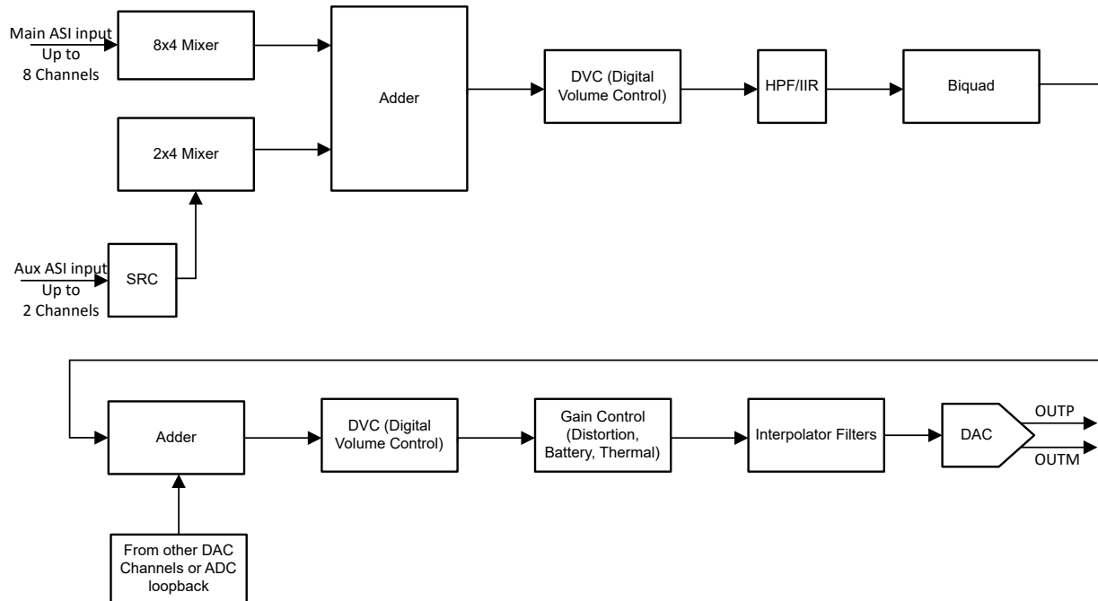
図 6-62. DAC Signal-Chain Processing Flowchart
