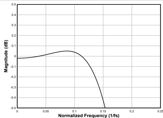
図 6-41. Linear-phase Decimation Filter Pass-Band Ripple
