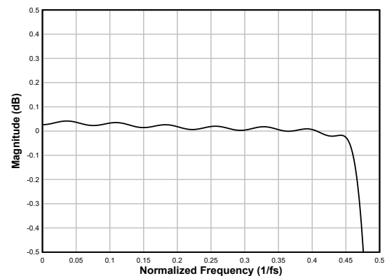
図 6-25. Linear-phase Decimation Filter Pass-Band Ripple
