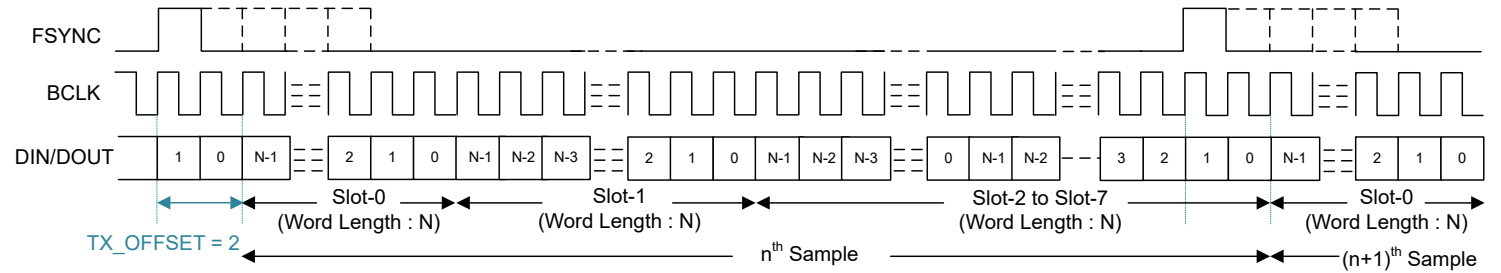
図 6-4. TDM Mode Protocol Timing (No Idle BCLK Cycles, PASI_TX_OFFSET = 2)
