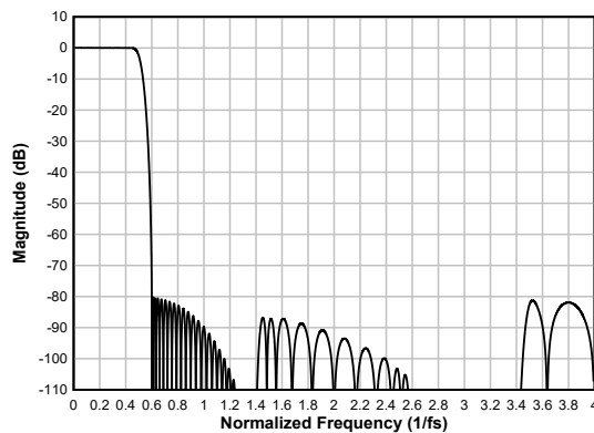
図 6-24. Linear-phase Decimation Filter Magnitude Response
