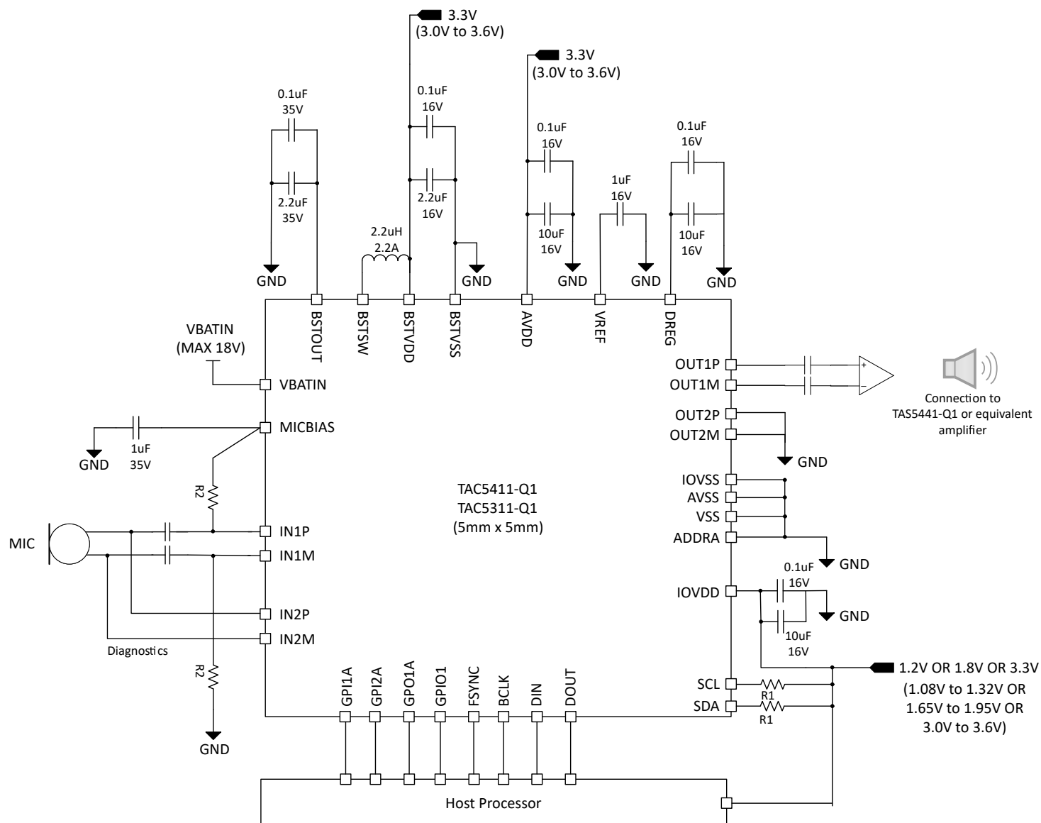
図 8-1. Mono Microphone with Mono Lineout Block Diagram
