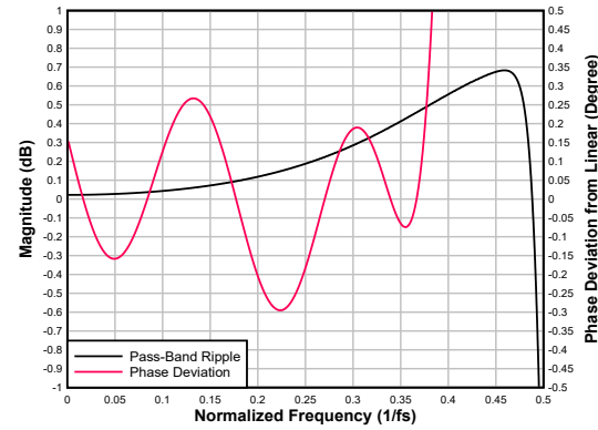
図 7-30. Low-latency Decimation Filter Pass-Band Ripple and Phase Deviation
