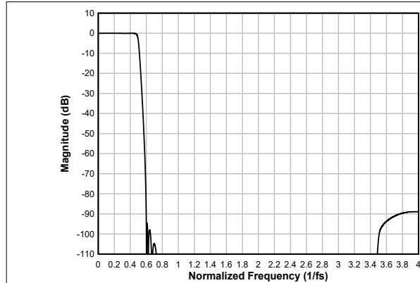
図 7-54. Low-latency Interpolation Filter Magnitude Response
