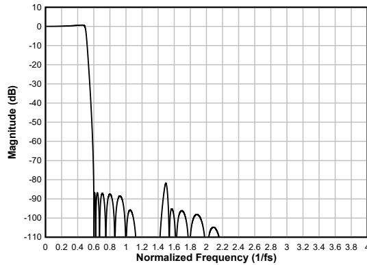
図 7-29. Low-latency Decimation Filter Magnitude Response
