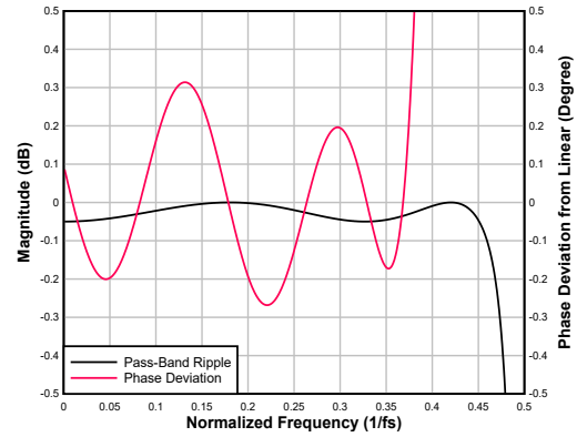
図 7-61. Low-latency Interpolation Filter Pass-Band Ripple and Phase Deviation
