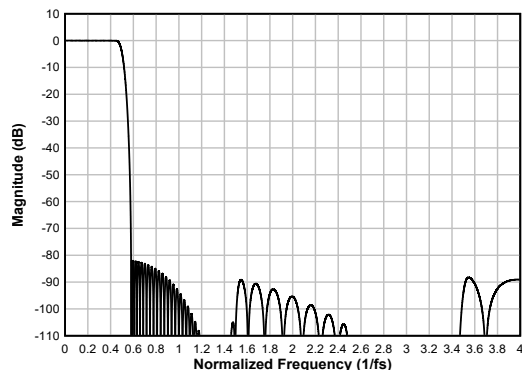
図 7-40. Linear Phase Interpolation Filter Magnitude Response
