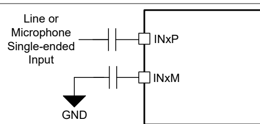
7-16. Single-Ended AC-Coupled Input Connection
