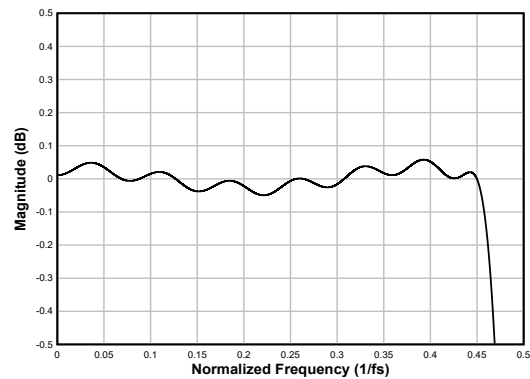
図 7-29. Linear Phase Decimation Filter Pass-Band Ripple
