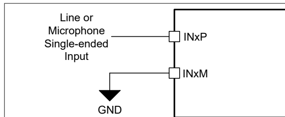
7-15. Single-Ended DC-Coupled Input Connection
