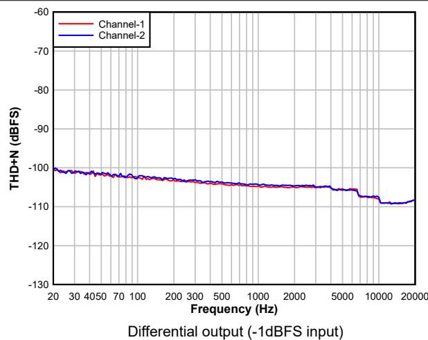
図 6-25. DAC THD+N Level vs Frequency
