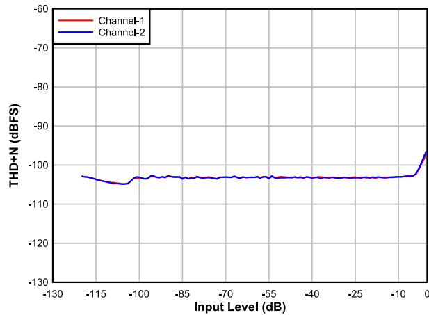
図 6-5. ADC THD+N Level vs Input
