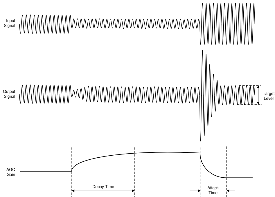
図 7-68. AGC Characteristics
