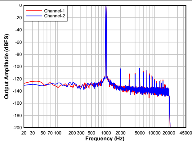
図 6-29. DAC FFT with Idle Channel Input
