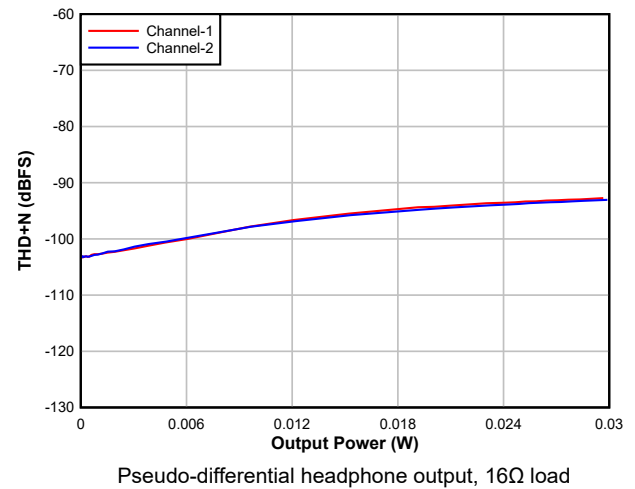
図 6-24. DAC THD+N Level vs output power
