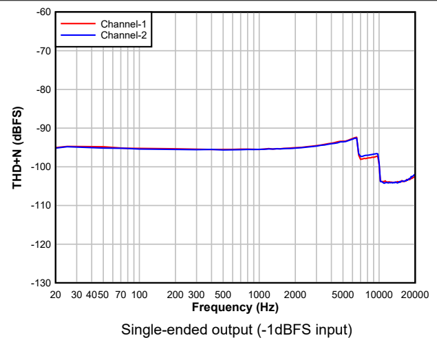
図 6-26. DAC THD+N Level vs Frequency
