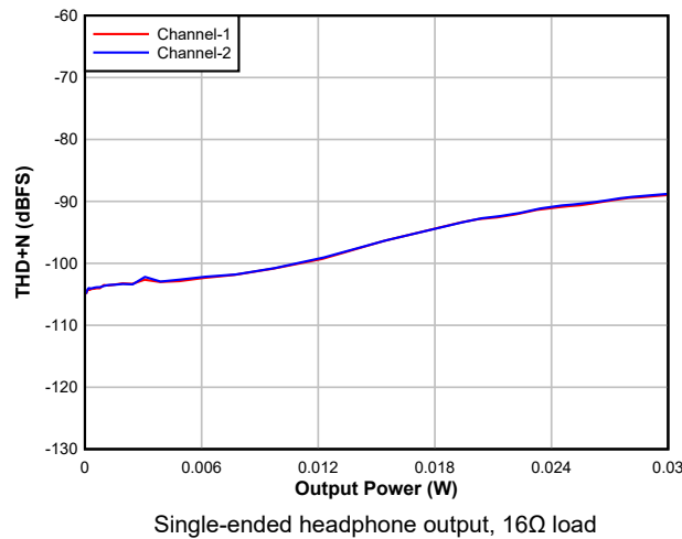
図 6-23. DAC THD+N Level vs output power
