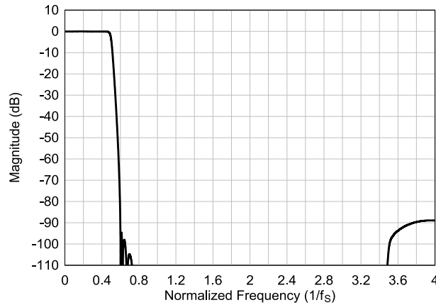
図 7-99. Ultra-Low-Latency interpolation Filter Magnitude Response
