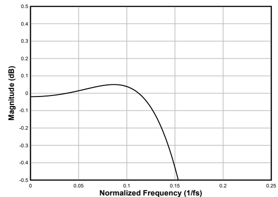
図 7-47. Linear-phase Decimation Filter Pass-Band Ripple
