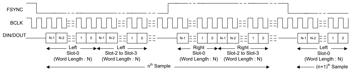
図 7-9. I 2 S Protocol Timing (PASI_TX_OFFSET = 0 and PASI_BCLK_POL = 1)
