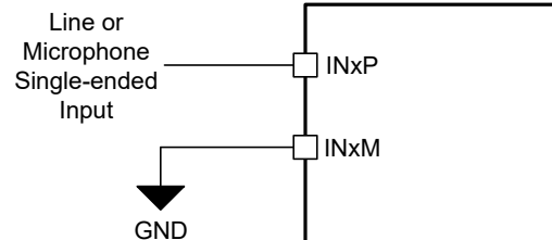
図 7-18. Single-ended DC-Coupled Input Connection (ADC_CHx_INSRC set to 2'b01 and ADC_CHx_CM_TOL set to 2'b01 or 2'10)
