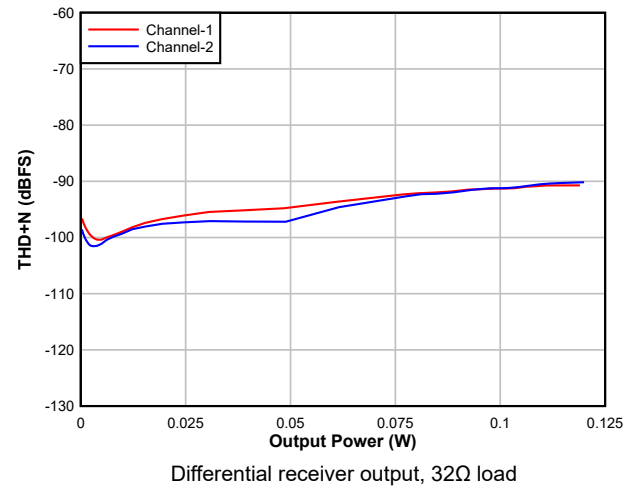
図 6-22. DAC THD+N Level vs output power
