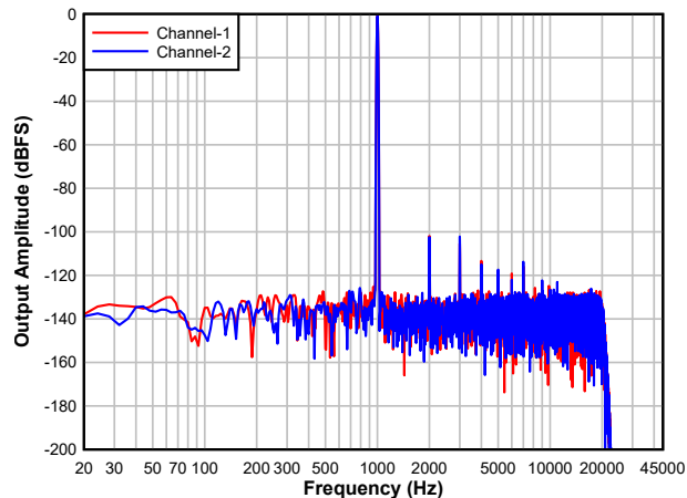
図 6-16. ADC FFT with -1dBFS Input
