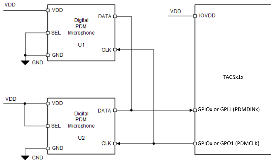
図 7-25. Digital PDM Microphones Connection Diagram for the TAC5112
