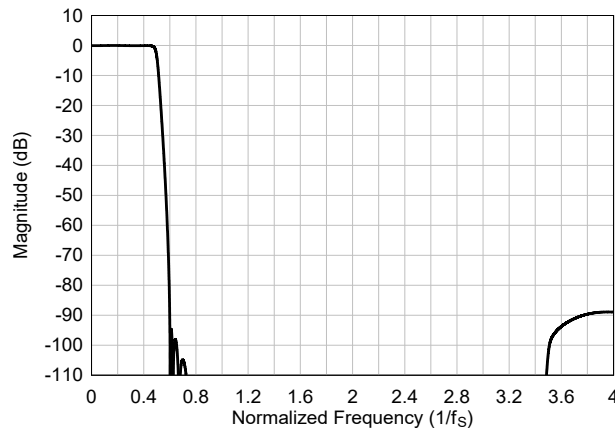
図 7-101. Ultra-Low-Latency interpolation Filter Magnitude Response
