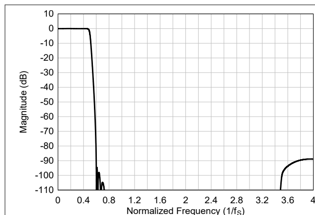
図 7-103. Ultra-Low-Latency interpolation Filter Magnitude Response
