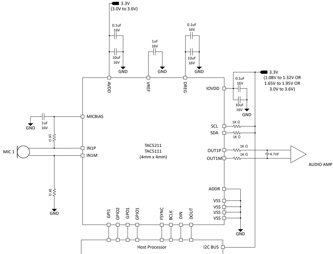
図 9-1. Mono Microphone with Mono Lineout Block Diagram
