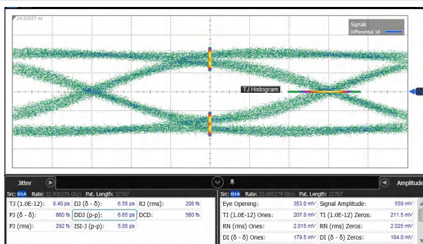
図 5-6. Through SN75LVPE5421 (6.5dB loss and DUT EQ=0)
