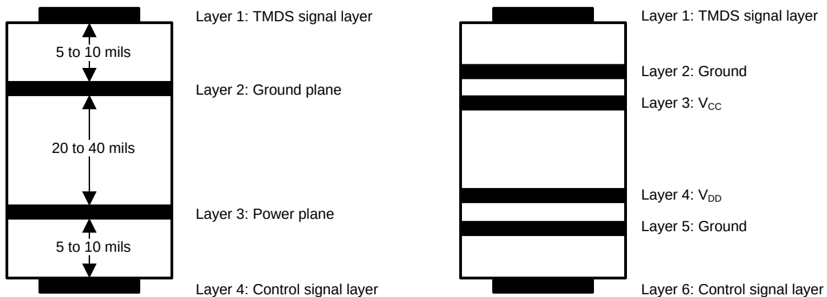
✎ 35. Recommended 4- or 6-Layer Stack for a Receiver PCB Design
