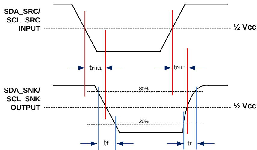
FIG 17. DDC Propagation Delay – Source to Sink
