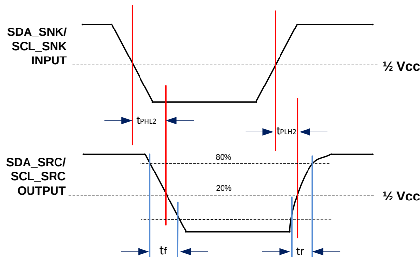
FIG 18. DDC Propagation Delay – Sink to Source
