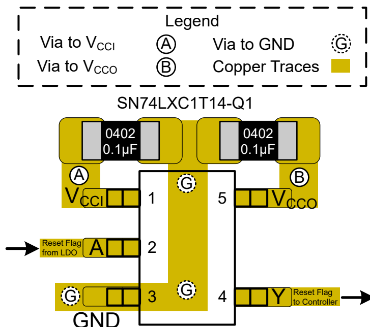
FIG 11-1. Layout Example – SN74LXC1T14-Q1
