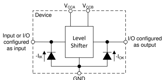
図 8-2. Electrical Placement of Clamping Diodes for Each Input and Output
