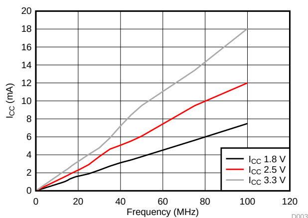
FIG 13. I_{CC} vs Frequency
