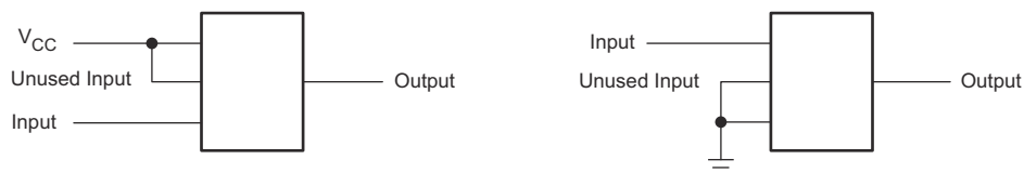
§ 15-1. Layout Diagram
