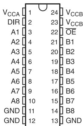
図 5-1. PW Package, 24-Pin TSSOP (Top View)
