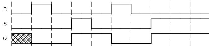
図 8-2. Application Timing Diagram
