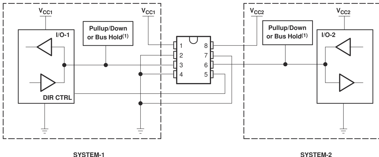
図 8-2. Bidirectional Logic Level-Shifting Application
