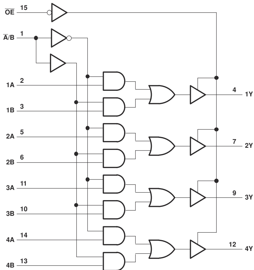
図 6-1. Logic Diagram (Positive Logic)
