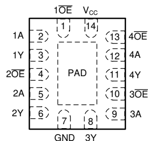
図 3-2. BQA Package, 14-Pin WQFN (Top View)
