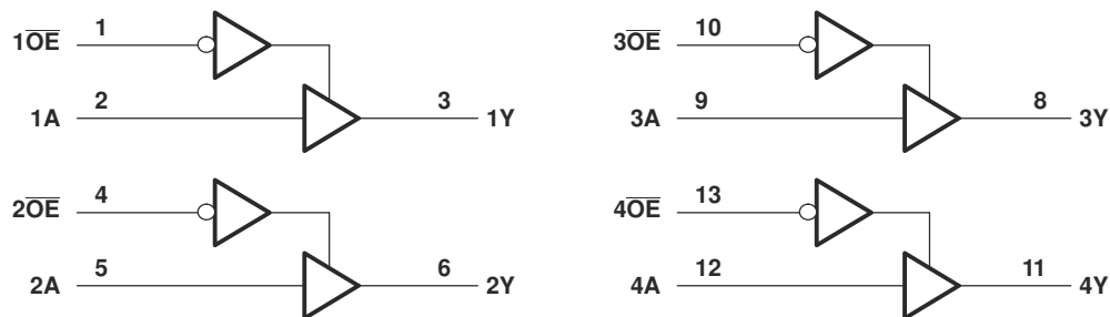
図 6-1. Logic Diagram (Positive Logic)
