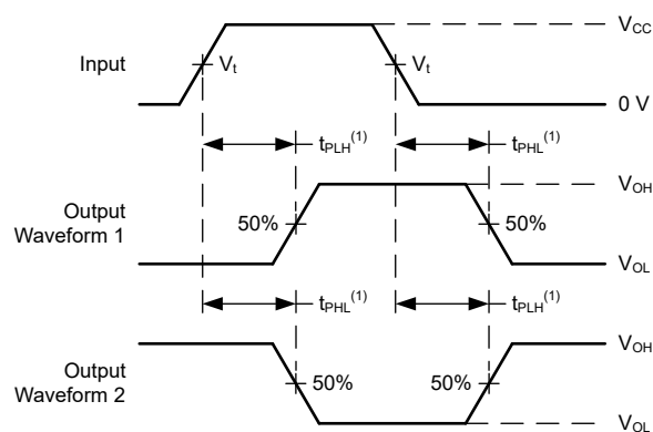
FIG 6-2. Voltage Waveforms Propagation Delays
