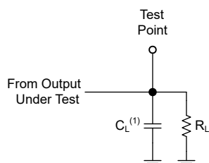
FIG 6-1. Load Circuit for Push-Pull Outputs
