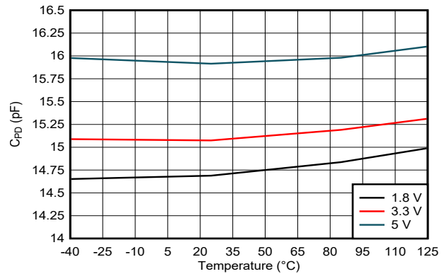
FIG 6-4. Power Dissipation Capacitance per Gate Across Temperature, 1.8-V, 3.3-V, and 5-V Supply
