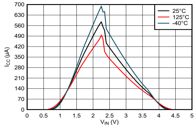
FIG 6-2. Supply Current Across Input Voltage, 5-V Supply
