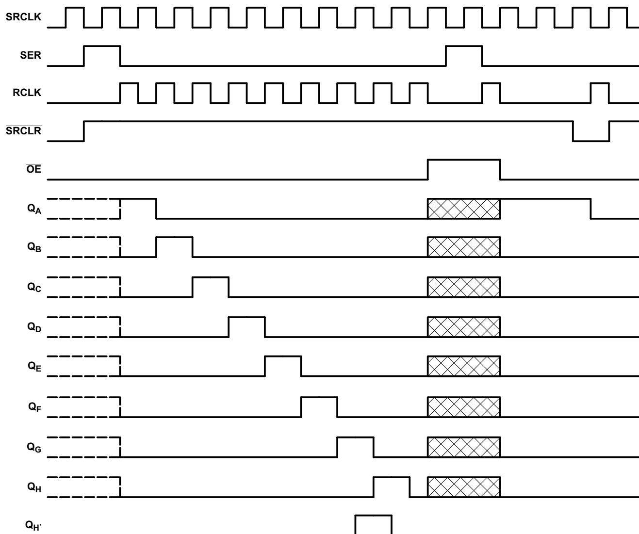
6-1. Timing Diagram
