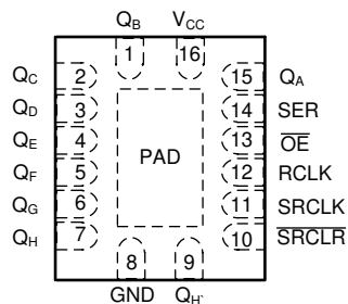
図 5-2. WBQB Package, 16-Pin WQFN Transparent (Top View)
